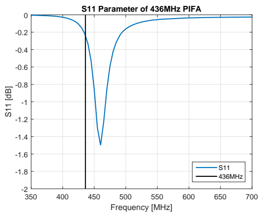
Figure 5: Reflection coefficient of the first antenna design.
