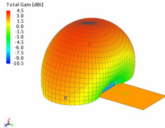
Figure 12: Far field radiation pattern of the PIFA at its resonance frequency.
