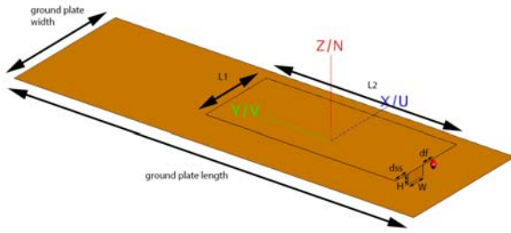
Figure 3: Structure of the PIFA.
