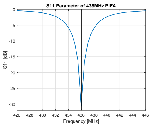
Figure 11: Reflection coefficient of the PIFA antenna.
