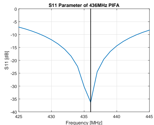
Figure 6: Return loss of the second antenna design.
