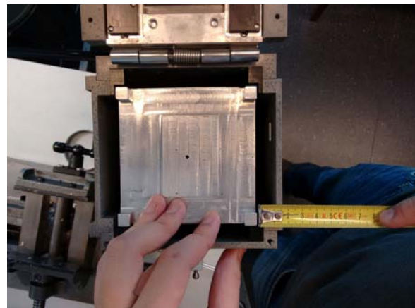
Figure 2: Dummy 3U CubeSat in a launch POD showing the space available for the patch to stick out. [Credit: Jan Verwilligen]
