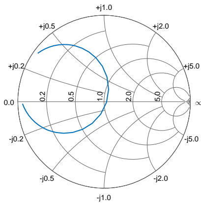
Figure 9: Smith chart of the complex reflection coefficient of the PIFA antenna.
