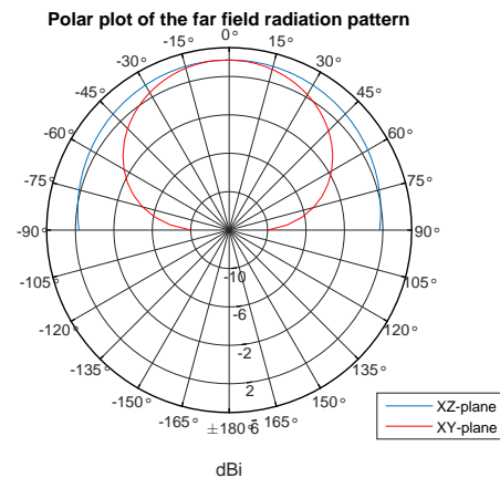
Figure 13: Polar plot of the far field radiation pattern of the PIFA at its resonance frequency.
