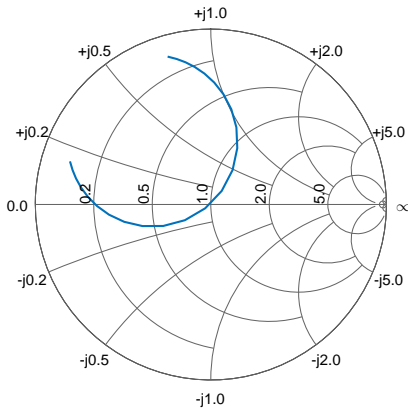
Figure 7: Smith chart plotting the complex return loss of the second antenna design.
