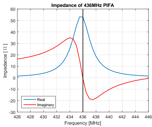
Figure 10: Real and imaginary impedance of the PIFA antenna.
