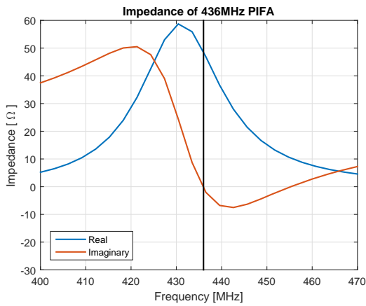
Figure 8: Impedance plot of the second antenna design.
