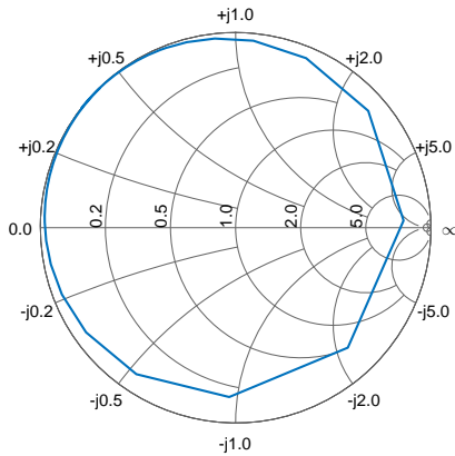
Figure 4: Smith chart with the complex S11 reflection coefficient of the first antenna design.
