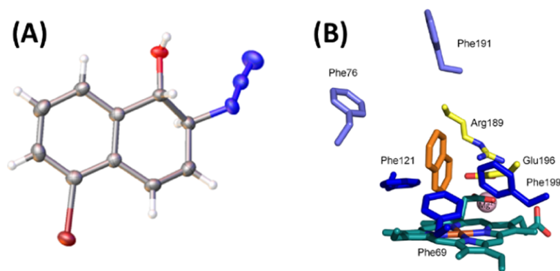
Figure 1. Crystal structure of (1 S ,2 S )-2-azido-5-bromo-1,2-dihydronaphthalen-1-ol (A) obtained from the PaDa-I-catalyzed epoxidation of 1-Br-naphthalene followed by nucleophilic ring opening with NaN 3 . (B) Active site model of PaDa-I in complex with naphthalene presenting the pro-( R )-face compound I. Naphthalene is placed between Phe121 and Phe199 in a T-packing mode with strong hydrophobic interaction with Phe69 that maintains a highly conserved orientation. Dark blue: Phe triad orienting the substrate, yellow: acid–base pair, and light blue: Phe pair involved in the guidance of the substrate to the active site.
