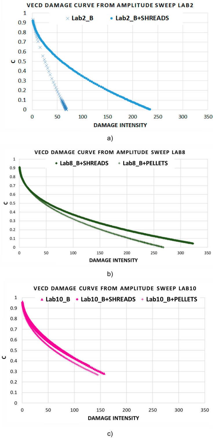
Figure 26. C-Damage Intensity: (a) Lab2, (b) Lab8 and (c) Lab10.
