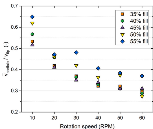
Fig. D.1. Supporting information for Section 3.2 demonstrating the influence of the fill level and rotation speed on the ratio of the mean particle velocity to the impeller blade tip speed. The data was acquired from an additional extended experimental data set, comprising a larger number of experimental conditions.
