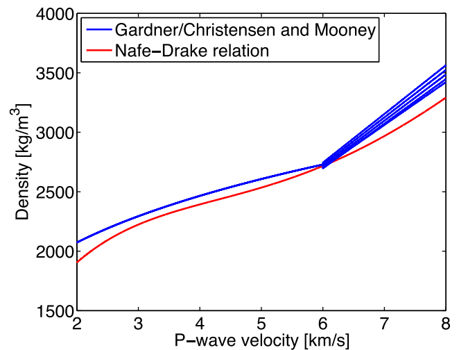
Figure 3. The relation between crustal density and P -wave velocity according to two studies. The red line shows the Nafe–Drake relationship (Ludwig et al. 1970) and the blue line shows the Gardner rule for sedimentary rocks, complemented by empirical relations of Christensen & Mooney (1995) for crustal rocks, which are depth dependent.
