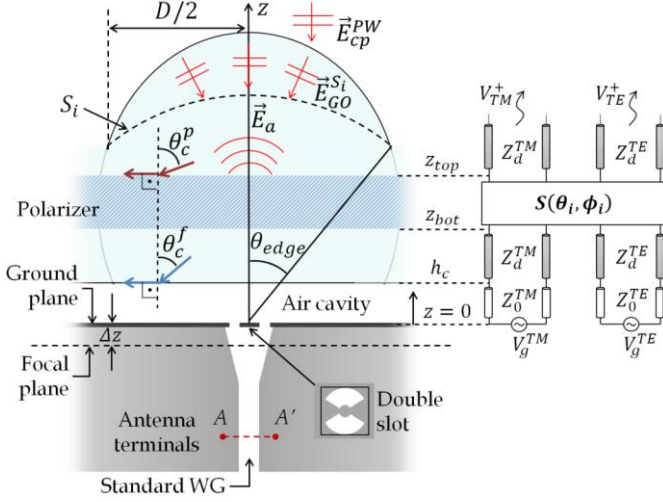
Fig. 3. Left: Main parameters of the elliptical lens geometry with integrated polarizer, and LW feeder. Optimized values: h_c = 0.56\lambda_0 , z_{bot} = 2.27\lambda_0 , z_{top} = 6.53\lambda_0 , \theta_{edge} = 40\text{deg} , \Delta z = -2.8\text{mm} . The fields used for the lens aperture efficiency and axial ratio calculation are as well represented here ( \vec{E}_a , \vec{E}_{GO}^{Si} and \vec{E}_{cp}^{PW} ). Right: Equivalent transmission line model applied for the CP primary pattern calculation.
