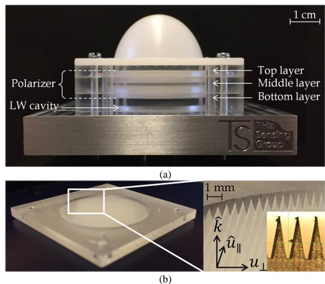
Fig. 1. a) CP antenna prototype. From bottom to top: split-block waveguide, integrated polarizer in Topas material and lens fabricated with HDPE. b) Bottom polarizer layer and side view of the polarizer pyramidal gratings.
