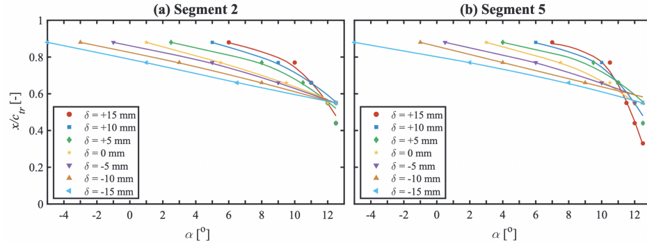
Figure 13. Location of the transition point versus angle-of-attack for various morphing flap settings for (a) flap segment 2 (inboard) and (b) flap segment 5 (outboard) [36].
