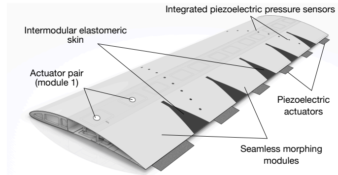
Figure 10. SmartX-Alpha sensor hardware integration.
