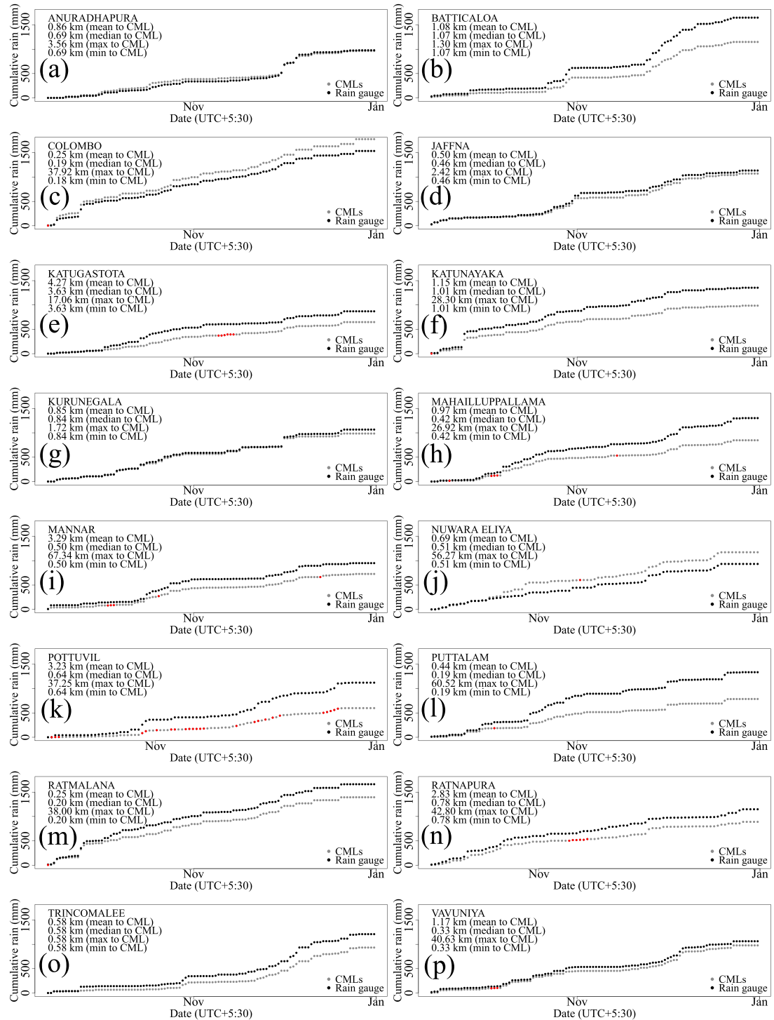
Figure 3. (a)–(p) Cumulative rainfall depths. Comparison of commercial microwave link (CML) based daily interpolated rainfall depths at the locations of gauges from the Sri Lanka Department of Meteorology which report daily rainfall depths. The red dots indicate the days for which the maximum distance of the underlying 15 min data to the nearest link antenna is larger than 5 km, and hence could have been large during rainfall.
