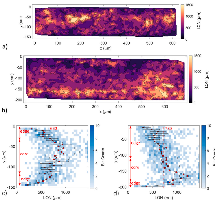
Fig. 9. Contour plot of length of neighbourhood (LON) for a) Tape A, b) Tape B; thickness profile for c) Tape A, d) Tape B. The dashed line represents the median calculated over the full cross-section, which value is noted at the top of each graph. For each horizontal bin, the median of the distribution is represented with red squares. The error bars represent the interquartile range. (For interpretation of the references to colour in this figure legend, the reader is referred to the Web version of this article.)
