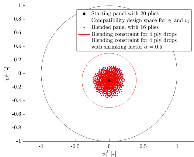
Fig. 4 Example of a 20-ply panel with all its possible blended adjacent panels 4 ply drops. Blending constraints without and with shrinking factor are shown in red and blue respectively. Original figure from Macquart et al. (2016a)
