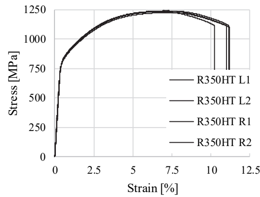
Figure 1: Monotonic engineering stress-strain curves, [15].
