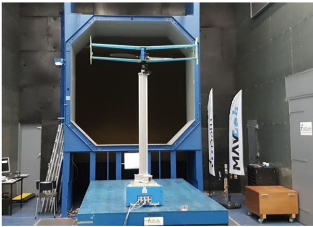
FIGURE 16 DelftaCopter in the Open Jet Wind tunnel of TUDelft. The tunnel outlet measures 2.85 \text{ m} \times 2.85 \text{ m} and can reach 30 \text{ m/s} wind speeds. DelftaCopter was mounted on a 1.8\text{-m} aluminum pole, which was standing on a force and moment balance. The Y-axis of the balance points into the tunnel opening. The X-axis points right in the picture and the Z-axis up
