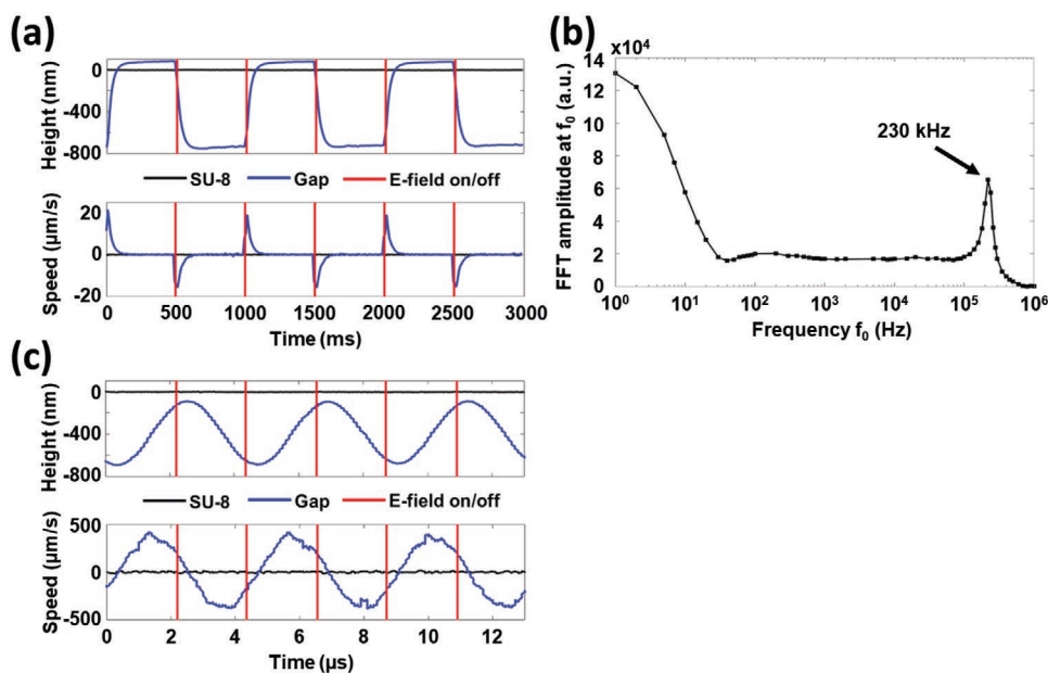
Figure 4. DHM measurements from electric field induced surface vibrations. a) The change in surface height and deformation speed using an AC potential of 150 Vpp at a frequency of 1 Hz. The gap distance is 100 \mu\text{m} . Vertical red lines indicate the moments the electric field switches on or off. b) Amplitude of the Fourier coefficient of each measured signal at f = f_0 . c) The change in surface height and deformation speed using an AC potential of 150 Vpp at a frequency of 230 kHz.
