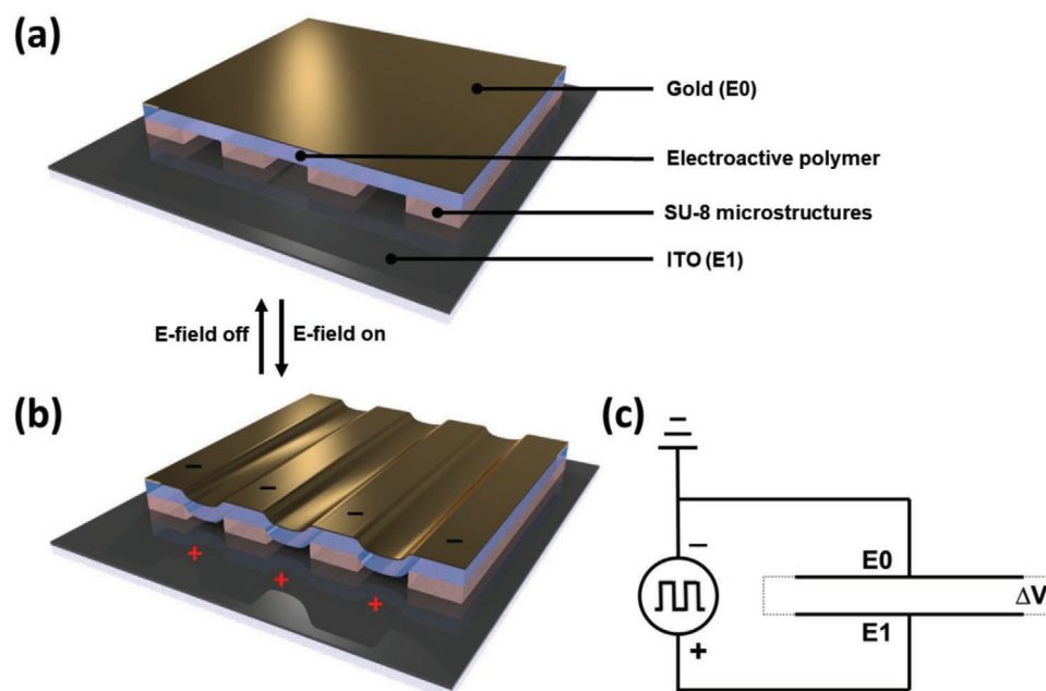
Figure 1. Design principle of an electroactive polymer coating with switchable surface topography. a) Schematic representation of the device configuration. b) After application of the electric field, the surface can alter its topography according to the programmed SU-8 structure underneath. As the pockets collapse, their content is pushed out of the sample via escape points at the edges of the samples. c) The electric circuit of the device. The electroactive polymer combined with the micro-structured SU-8 work as a two-plate capacitor when placed in the external electric field.
