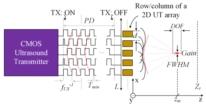
Fig. 2. 2D ultrasound phased array transmitter: properties of transducer driving signals, transducer array and focused ultrasound waves.
