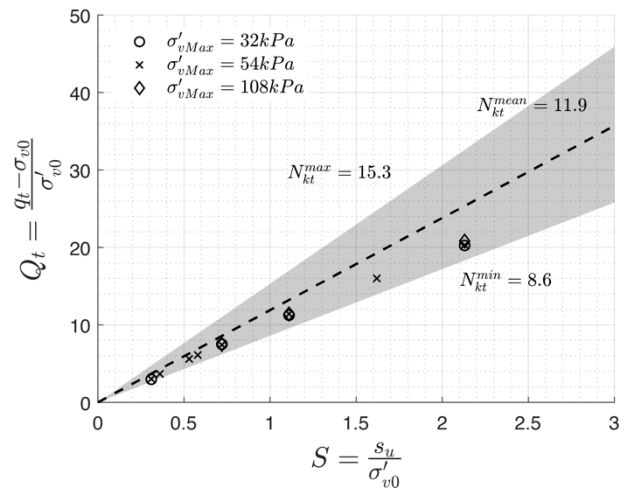
Figure 5. Evolution of normalised q_{net} with normalised s_u .
