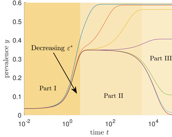
Figure 2.2: Plateau-behaviour in the Markovian \varepsilon -SIS process on the complete graph. Each curve is computed using the exact solution (2.5) and the parameters are N = 30 nodes, effective infection rate \tau = 2.5\tau_c^{(1)} = 2.5/(N-1) , the process starts with a single infected node and the effective self-infection rate \varepsilon^* = \{10^{-2}, 10^{-3}, 10^{-4}, 10^{-5}, 10^{-6}, 10^{-7}, 0\} . For \varepsilon^* \leq 10^{-5} , the background colours indicate the current phase of the \varepsilon -SIS process: (I) initial phase, (II) metastable behaviour and (III) convergence to the steady state.
