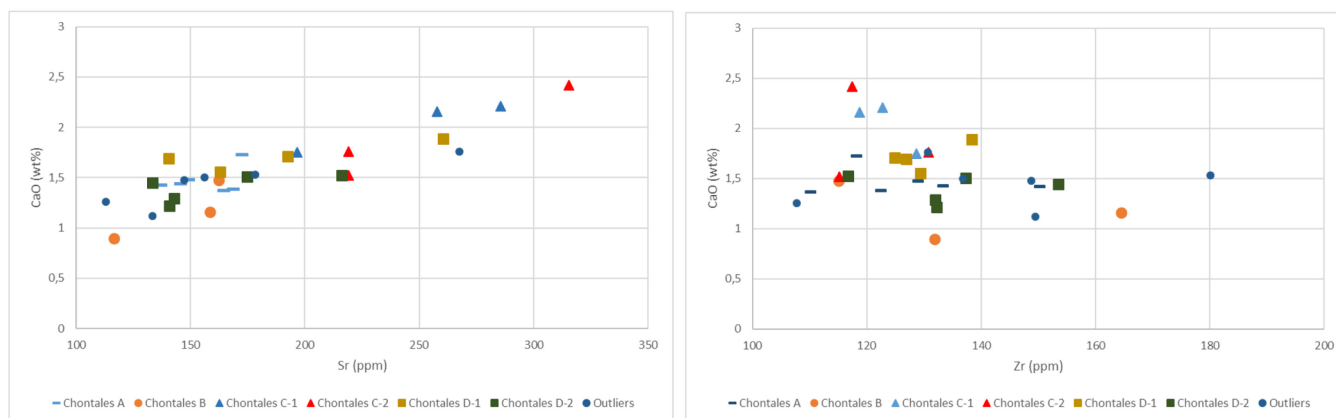
Fig. 3. Biplot of CaO (wt%) vs. Sr (ppm), CaO (wt%) vs. Zr (ppm) values of the archaeological ceramics from Aguas Buenas MI. Samples are coloured according to the results of the petrographic analysis.
