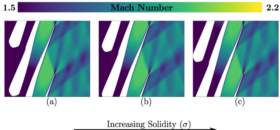
Fig. 8. Mach number contours of vanes operating with Toluene for \beta_{t1} = 6.0 and M_a = 2.0 with increasing \sigma from left to right: (a) 1.50, (b) 1.75 and (c) 2.00.
