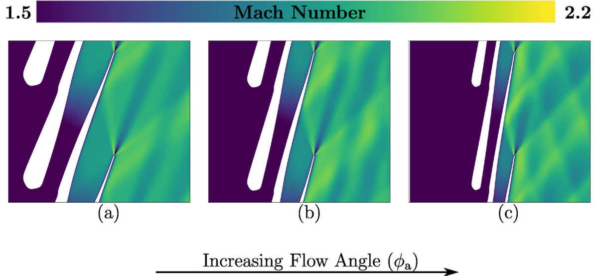
Fig. 10. Mach number contours of vanes operating with Toluene at \beta_{t1} = 6.0 and with increasing design flow angle from left to right: (a) 71^\circ , (b) 76^\circ and (c) 81^\circ .
