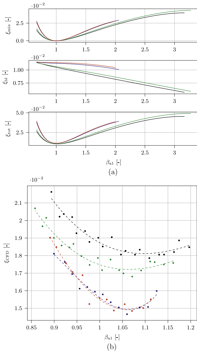
Fig. 4. Variation of \xi with \beta_{a1} for stator vanes operating with \beta_{t1} = 6.0 and \varphi_a = 70^\circ and with air (---), CO 2 (- - -), toluene (- · - ·) and MM (- - -) as working fluid. (a) trend lines obtained with the analytical method, (b) trend lines obtained with the CFD-based method. The dots in (b) represent the values obtained from CFD simulations at discrete intervals of \beta_{a1} and the dashed lines are trend lines obtained by fitting the dots with a cubic functional form.
