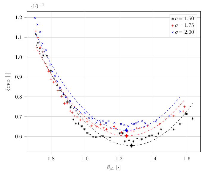
Fig. 7. Variation of \xi_{CFD} with \beta_{a1} for solidity ( \sigma ) of 1.50, 1.75 and 2.0, for \beta_{t1} = 6 and \phi_a = 71^\circ . The values corresponding to the scattered points are calculated from the results of CFD simulations, while the dashed lines are the hypothetical trends obtained by cubic fitting. The diamond on the dashed line shows the representation of the estimation of the value of \beta_{a1} that minimizes \xi_{CFD} .
