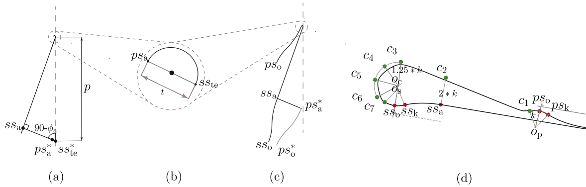
Fig. 2. Schematic representation of the graphic procedure to obtain the geometry of an axial supersonic vane, (a) semi-bladed region, (b) trailing edge (c) diverging-nozzle section and (d) converging section.
