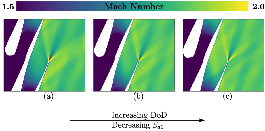
Fig. 5. Mach number contours of vanes operating with Toluene as working fluid for \beta_{t1} = 6.0 and \phi_a = 71^\circ . From left to right: (a) \beta_{a1} > \beta_{opt,a1} , (b) \beta_{a1} = \beta_{opt,a1} and (c) \beta_{a1} < \beta_{opt,a1} .
