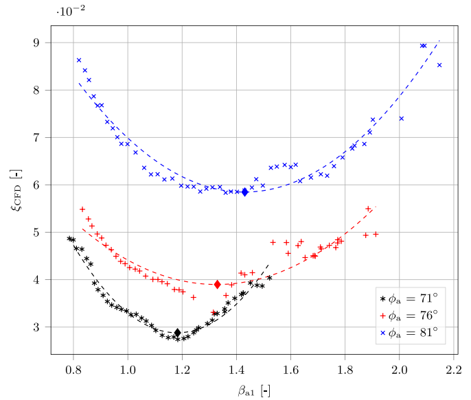
Fig. 9. Variation of \xi_{CFD} with \beta_{a1} for \varphi_a of 71^\circ , 76^\circ and 81^\circ . The scattered points represent results from individual CFD simulations while the dashed lines are the hypothetical trends obtained by cubic fitting of these points. The diamonds on the dashed lines highlight the estimation of the optimal value of \beta_{a1} .
