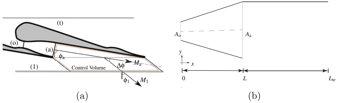
Fig. 1. Schematics of the nozzle geometries related to the analytical loss models: (a) geometry for the mixing loss model, showing Mach number, deviation angle and the different stations in the supersonic vane. The control volume is outlined in red. (b) illustration of the domain considered for the computation of the boundary layer losses. (For interpretation of the references to colour in this figure legend, the reader is referred to the Web version of this article.)
