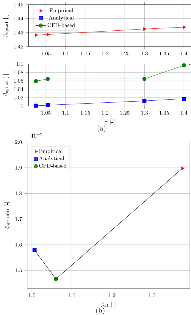
Fig. 6. Comparison of \beta_{opt,a1} obtained with the three design methods (a) Variation of \beta_{opt,a1} depending on the molecular complexity of the working fluid, and (b) \xi_{CFD} obtained by simulating \beta_{opt,a1} from the three methods with Toluene as the working fluid.
