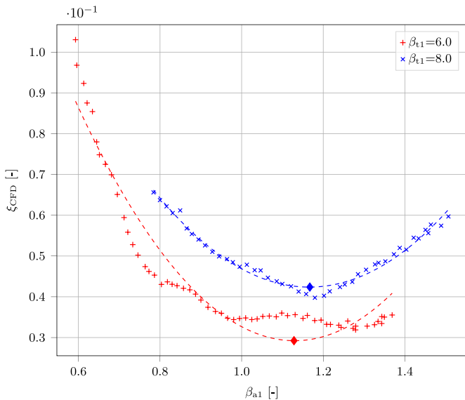
Fig. 11. Variation of \xi_{CFD} with \beta_{opt,a1} , for \beta_{t1} of 6.0 and 8.0. The scattered points represent values computed from CFD simulations while the dashed lines are the hypothetical trends obtained by cubic fitting. The diamonds on the dashed lines highlight the estimation of the optimal value of \beta_{a1} .
