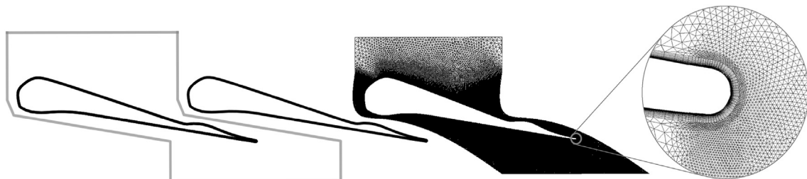
Fig. 3. Representation of the axial vane geometry. The boundary of the computational flow domain is outlined in gray (left). The discretized computational domain is also reported (right), together with the zoomed-in view of the trailing edge.
