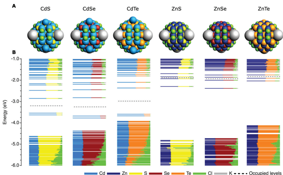
Figure 3.2. Effect of charging different \text{M}_{68}\text{X}_{55}\text{Cl}_{26} ( \text{M} = \text{Cd}, \text{Zn}; \text{X} = \text{S}, \text{Se}, \text{Te} ) zincblende NCs on their structure and DOS. (A) Structure and (B) DOS of the NCs when charged with four electrons. The total system is kept neutral by the addition of a potassium cation for each added electron. The structure and DOS of the uncharged NCs are given in Figure A3.4.
