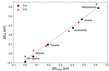
Figure 5.5. Correlation between \Delta E_R and \Delta E_{\text{bind}} for electron charged CdSe QDs with different ligands binding directly to Cd 1 and Cd 2 , as determined with the reduction of Cd 1 (black circles) and Cd 2 (red triangles). The gray dashed line is a linear fit to the data points.
