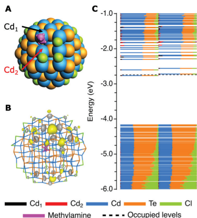
Figure 3.4. Influence of methylamine on the formation of Cd–Cd dimers. (A) Structure of the NC when a Cl 0 is replaced by a methylamine ligand (this is isoelectric to removing a chloride and injecting one extra electron into the NC). (B) Contour plot of the HOMO level of the NC, indicating that the electron is delocalized over the NC. (C) DOS of the NC, showing a clean bandgap and one electron in the CB.
