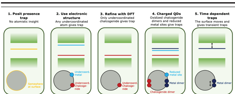
Figure 1.2. Five levels of describing trap states. Level 1: the presence of a trap state is posited; its atomistic origins are not specified. Level 2: based on the QD electronic structure, each undercoordinated atom is assumed to give a trap state. Level 3: DFT calculations show that only undercoordinated chalcogenide atoms give a trap. Level 4: Charge unbalanced QDs can give rise to in-gap states not present in charge balanced QDs, like reduced metal sites and chalcogenide dimers. Level 5: the QD surface is continually in motion, leading to the dynamic formation and disappearance of trap states.
