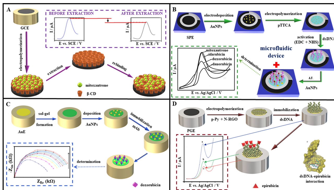
Figure 5. (A) The GCE modified with MIP sensor based on \beta -CD for mitoxantrone detection. Voltammograms were reprinted from [246] with permission from Elsevier; (B) The steps of the preparation of a microfluidic device, which integrated pre-concentration, separation, and simultaneous detection of doxorubicin, daunorubicin, idarubicin, and mitoxantrone by utilizing electrokinetic separation and electrochemical detection method, using amperometric biosensors based on a modified SPE. Voltammograms were reprinted from [249] with permission from Elsevier; (C) The schematic representation of AuE modified with sol-gel functionalized with thiol functional groups, AuNPs, and mAb for the doxorubicin impedimetric detection. EIS spectra reprinted from [264] with permission from Elsevier; (D) The PGE modified with dsDNA, N-RGO, and p-Py for indirect detection of epirubicin. Voltammograms were reprinted from [269] with permission from Elsevier.
