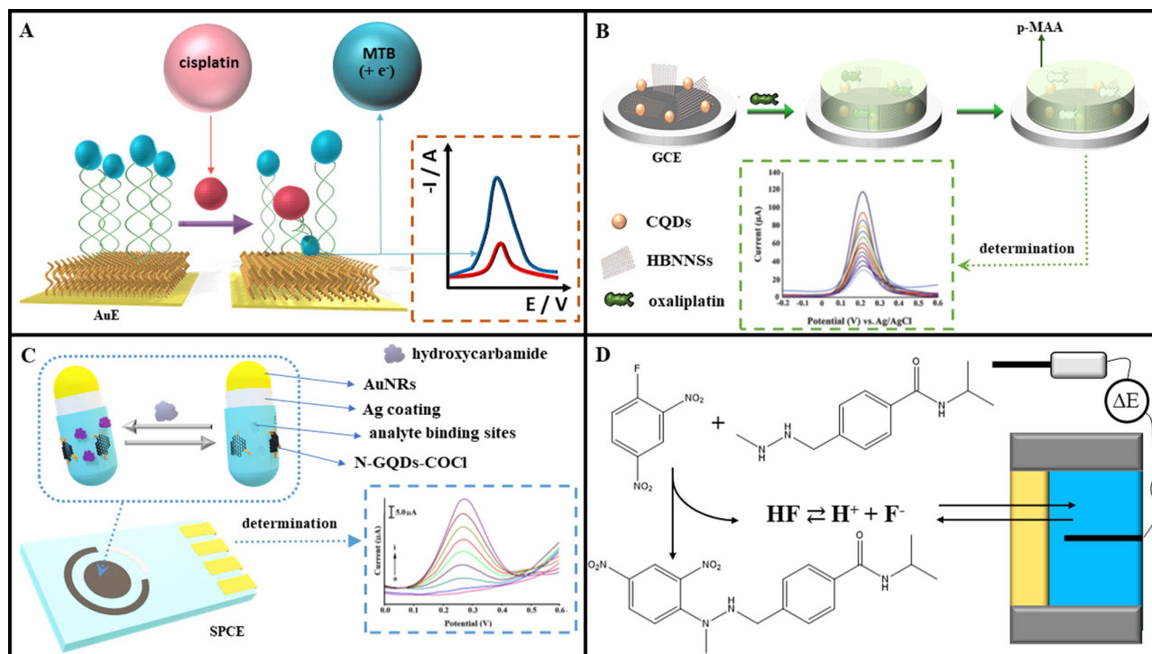
Figure 7. (A) Cisplatin sensors constructed at the AuE surface modified with thiolated MTB-terminated DNA strands. The analytical signal originates from the DNA conformational changes triggered upon cisplatin (red sphere) binding. Prepared based on [400]; (B) Protocol for the oxaliplatin imprinting in a blend composed of CQDs, HBNNs, and Zr(IV)-MOF in a poly-methacrylic acid (p-MAA) MIP. DP voltammograms reprinted from [405] with permission from Elsevier; (C) SPCE decorated with a nanomaterial derived from gold NRs (AuNRs) further modified with Ag coating and N-GQDs-COCl containing MIP used for the hydroxycarbamide sensing. DP voltammograms reprinted from [408] with permission from Elsevier; (D) The scheme showing indirect, potentiometric detection of procarbazine using FISE. Fluoride ions are the side project of the procarbazine reaction with 1-fluoro-2,4-nitrobenzene reagent. Prepared based on [411].
