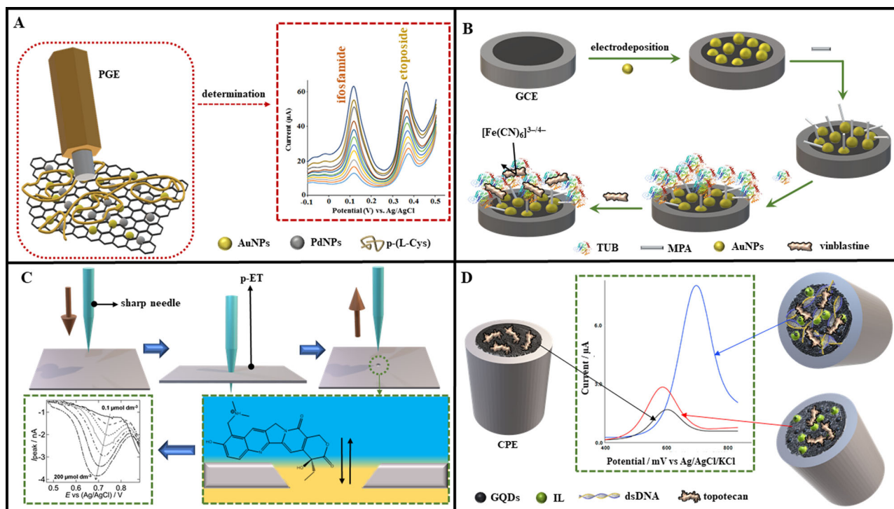
Figure 4. (A) Scheme depicting the PGE modified with RGO further decorated with AuNPs, PdNPs, and p-(L-Cys) used for the simultaneous determination of ifosfamide and etoposide. DP voltammograms reprinted from [199] with permission from Elsevier; (B) GCE surface sequential modification with AuNPs, MPA layer further used as the TUB anchor. The presented architecture was employed as the impedimetric vinblastine sensor. Prepared based on [209]; (C) Electrified liquid-liquid interface miniaturization protocol based on p-ET film micro punched with a sharp needle. Formed micro aperture served as the support for the soft junction. The signals recorded at the corresponding DP voltammograms originate from the topotecan simple interfacial ion transfer reaction. Voltammograms reprinted from [215] with permission from American Chemical Society; (D) Series of DP voltammograms for topotecan recorded at bare CPE (bottom left corner) and bulk-modified CPE with IL and GQDs (bottom right corner) and additionally decorated with dsDNA (upper right corner). DP voltammograms reprinted from [218] with permission from Elsevier.
