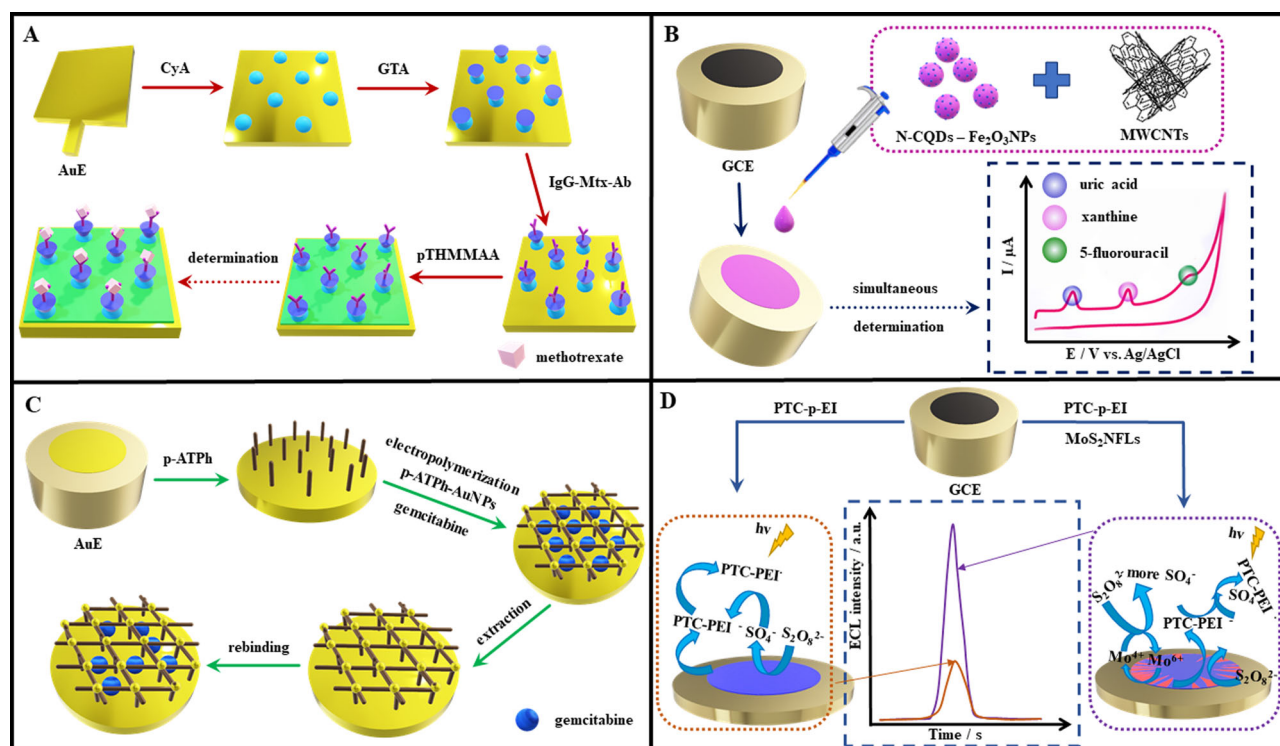
Figure 3. (A) The steps of the preparation of immunosensor based on AuE modified with cysteamine (CyA), glutaraldehyde (GTA) as a linker, immunoglobulin G methotrexate antibody (IgG-Mtx-Ab), and N-[tris(hydroxyl-methyl)methyl]acrylamide (pTHMMAA) to block pinholes. The immunosensor was used for the methotrexate sensing. Prepared based on [80] ; (B) Schematic representation of the GCE surface modification procedure with N-CQDs, Fe 2 O 3 NPs, and MWCNTs used for the simultaneous electrochemical detection of 5-fluorouracil, uric acid, and xanthine. Voltammograms reprinted from [101] with permission from Elsevier; (C) MIP sensor based on electropolymerized molecularly imprinted MOF used for the detection of gencitabine. The sensor was prepared by immersing the AuE in p-aminothiophenol (p-ATPh) solution, and further by electropolymerization of the aniline moieties of the aniline moieties of p-ATPh functionalized with AuNPs on AuE modified with p-ATPh in the presence of gencitabine as a template molecule. Prepared based on [142] ; (D) Molybdenum disulfide nanoflowers (MoS 2 NFLs) as signal-promoter of p-EI functionalized PTC and S 2 O 8 2- system for fabricating an electrochemiluminescence methotrexate sensor. Prepared based on [149] .
