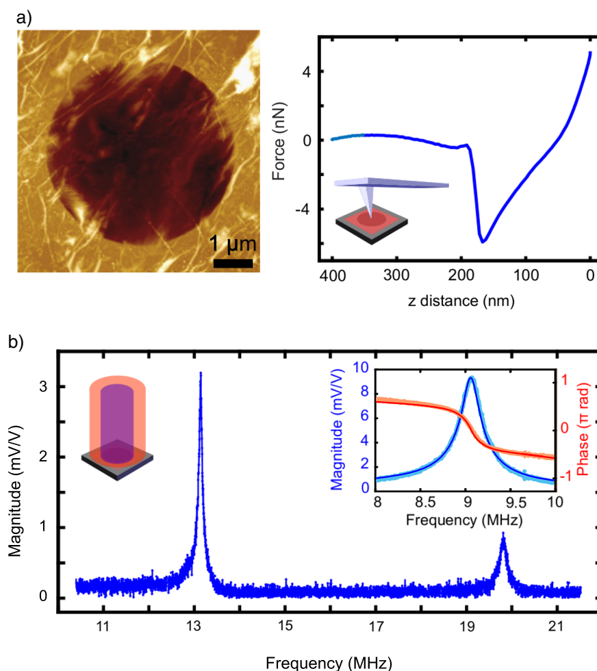
Fig. 3 Characterization of h-BN 5 \mu\text{m} in diameter drums. a AFM image of the h-BN drum showed in Fig. 1b. The CVD material shows wrinkles and sidewall adhesion as in CVD graphene ( left panel ). The force distance curve in the center of the drum is obtained by AFM indentation in Peak Force mode. From the retraction curve we extract the tension and Young's modulus. b Mechanical frequency spectrum of the same drum at room temperature and \sim 10^{-6} mbar when measured with the optical interferometric technique after cleaning. The second resonance peak appears around 1.5 times the fundamental frequency, indicating membrane behavior. 37 Inset Mechanical fundamental frequency and phase analysis of the same drum before cleaning. By fitting the frequency peak to the driven harmonic oscillator equation, we extract the tension values
