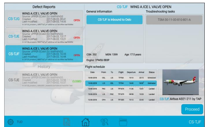
Figure 3: UI for selecting a defect.
