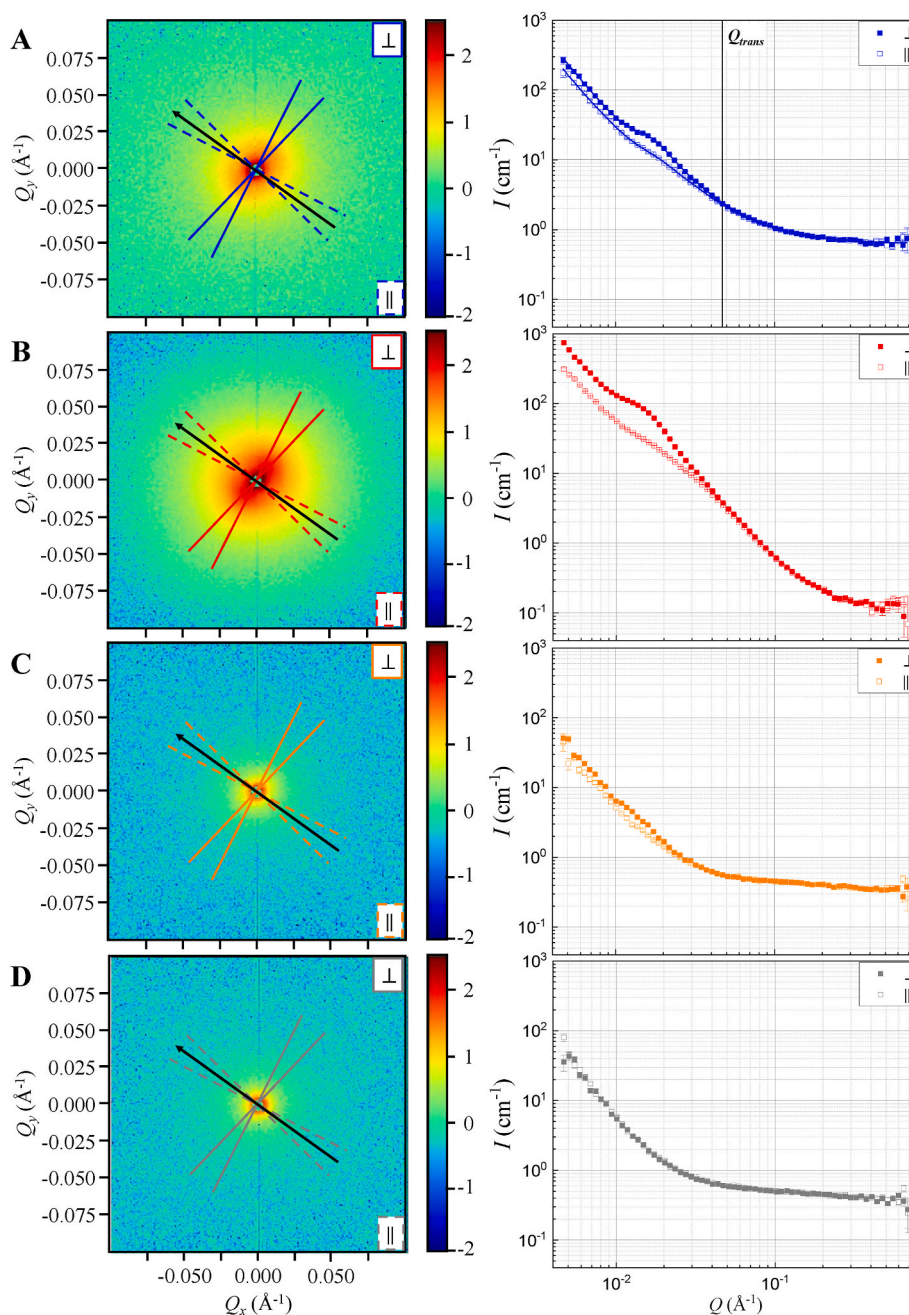
Fig. 5. 2D SANS data (scattering intensities are on logarithmic scales) (left) and sector averages taken in the directions parallel ( \parallel ) and perpendicular ( \perp ) to the shear (right) for extrudate skin slices: a) unsoaked, b) soaked in 100% D_2O , c) soaked in 35% D_2O , and d) soaked in 42.5% D_2O . Black arrows indicate extrusion direction. Lines in a) (right) represent the fit with the broad peak model to the 100% H_2O extrudate SANS data.
