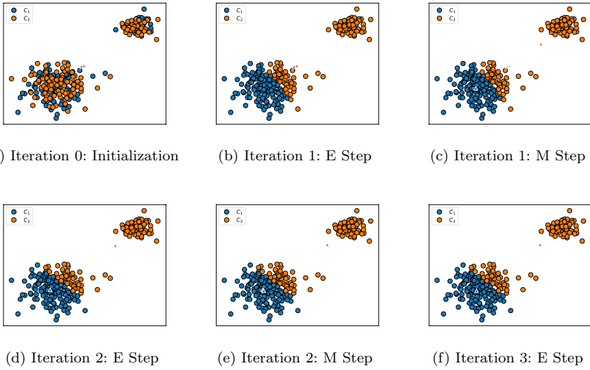
Fig. 10 Illustration of the k-means-based ESBG using X^* . The centroids are shown by the triangles of similar colors of their corresponding groups. The triangles of lighter colors represent the centroids in the previous iteration. (a): Initially, the data set is randomly and equally divided into two groups C_1 and C_2 , and the centroids of both groups are computed as the average of their group members. (b): In the E step of Iteration 1, each data point is assigned to the group whose centroid is nearer, while keeping the size of each group equal. (c): In the M step of Iteration 1, the centroid of each group is re-computed according to the new group structure updated in the last E step. (d)–(f): Successive iterations. The change in the positions of centroids from (d) to (e) is relatively small and can be observed when taking a closer look. The system has reached convergence since (f) .
