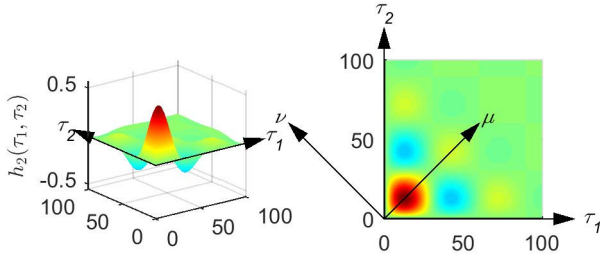
Fig. 3. Example of a function h_2(\tau_1, \tau_2) . The model corresponds to a Wiener-structure with a linear system followed by a square-operator. The left plot shows a 3D view of the model h_2 . The right plot shows the same model from a top view, with additionally an indication of the directions \mu and \nu , along which the smoothness and decay rate of the model were quantified during regularization. The colors of the surface indicate amplitude.
