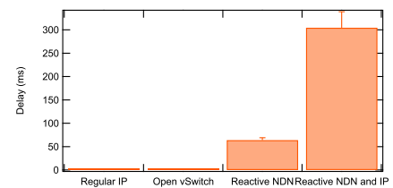
Fig. 4: Delay averages and 95% confidence interval.
