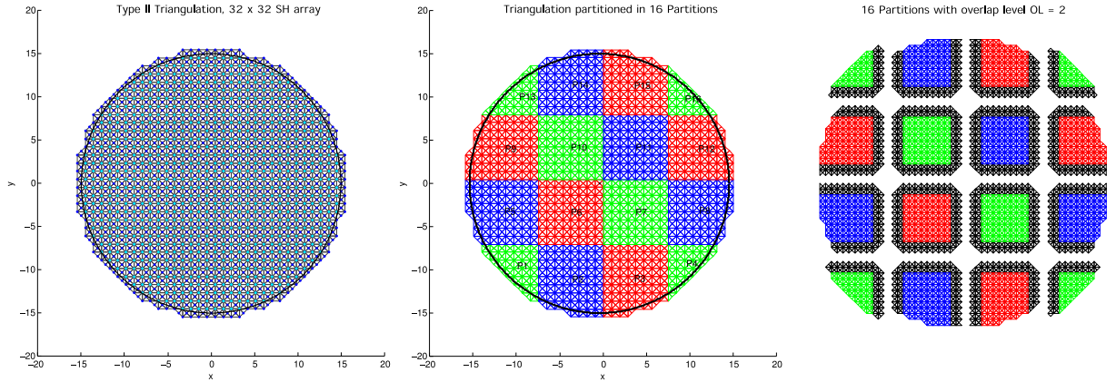
Fig. 8: Triangulation and partitioning example for D-SABRE. Left: Global Type II triangulation for a 32 \times 32 SH array constructed with vertices located on SH center locations (cyan) and added vertices (blue) to form the regular Type II triangulation and to cover the entire pupil domain. Center: Partitioning of the global triangulation in 16 partitions on a 4 \times 4 partition array. Right: Partitioning in 16 partitions with applied overlap level of OL=2 .
