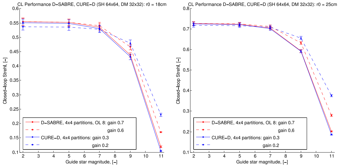
Fig. 10: Long exposure Strehl ratio comparing closed-loop performance and noise resilience of D-SABRE and CuRe-D for different of levels photon shot noise in a system with a 64 \times 64 SH array and a 32 \times 32 actuator array. Left: Turbulence with Fried parameter r_0 = 18\text{ cm} ; right: r_0 = 25\text{ cm} . A 4 \times 4 partitioning is constructed for both distributed methods. Two loop gains are considered for each method respectively optimized for low (solid) and high (dashed) noise levels. In the D-SABRE case OL = 64 / (2N_p) is used. The Strehl ratio is averaged for 10 turbulence realizations and plotted as a function of the guide star magnitude.
