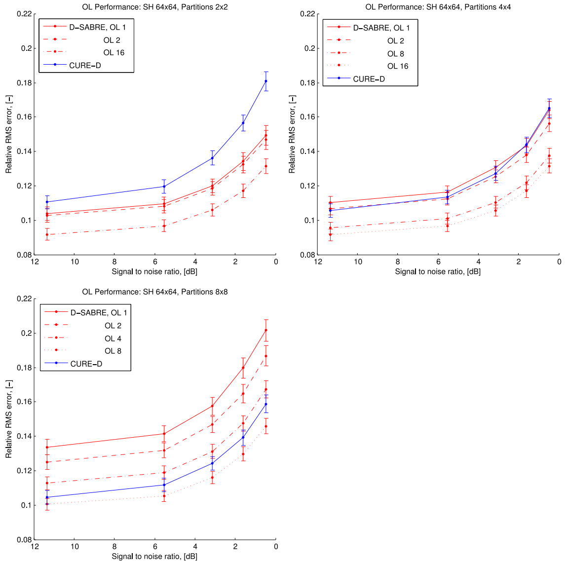
Fig. 9: Reconstruction accuracy and noise resilience for different levels of decomposition on a 64 \times 64 SH array of D-SABRE and CuRe-D . In the D-SABRE case different levels of partition overlap are considered. The average relative residual RMS is plotted as a function of signal to noise ratio.
