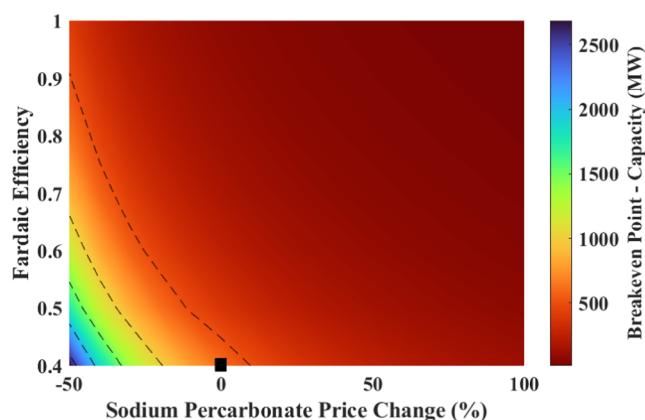
Figure 15. Effect of changes in the sodium percarbonate price and the Faradaic efficiency on the breakeven point (black marker shows the current situation).
