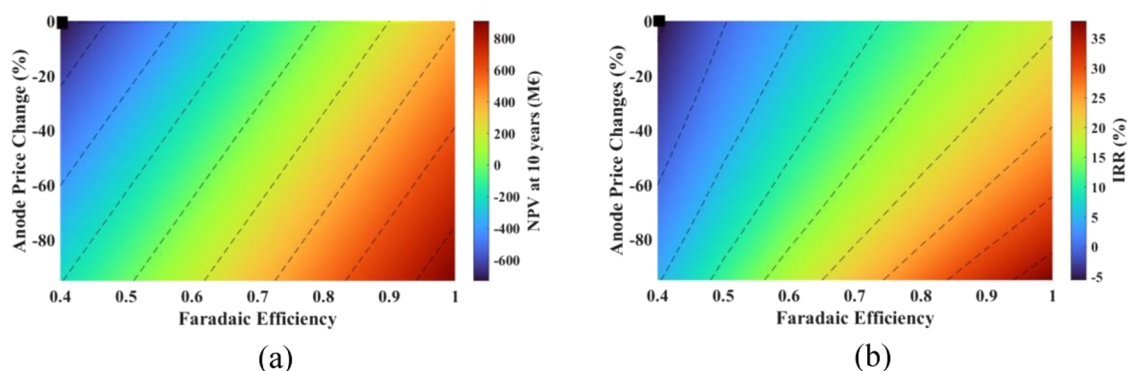
Figure 20. Effect of changes in Faradaic efficiency and the anode price on (a) NPV, and (b) IRR (black marker shows the current situation).
