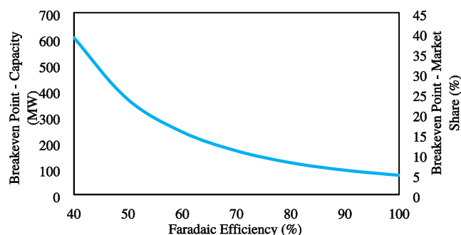
Figure 6. Effect of the Faradaic efficiency on the breakeven point.
