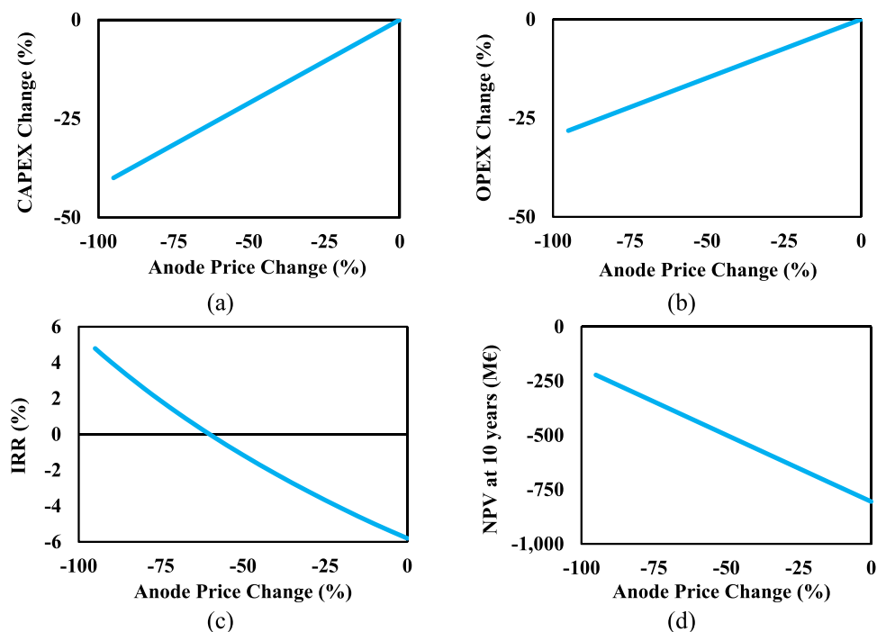
Figure 10. Effect of the anode price on (a) CAPEX, (b) OPEX, (c) IRR, and (d) NPV.
