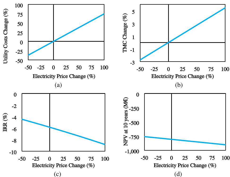
Figure 9. Effect of the electricity price on (a) Utility Costs, (b) TMC, (c) IRR, and (d) NPV.
