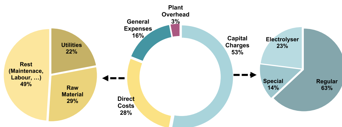
Figure 3. Cost review of the TMC.
