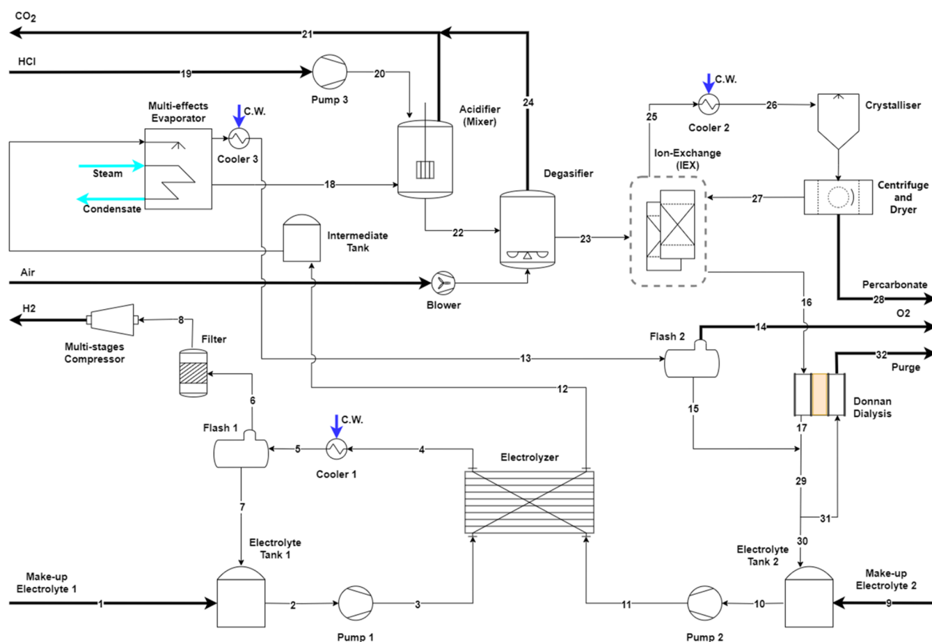
Figure 1. Process flow diagram of the proposed system. The catholyte recycles after a simple gas separation whereas the anolyte goes through a more complex chemical separation to extract SPC before recycling.
