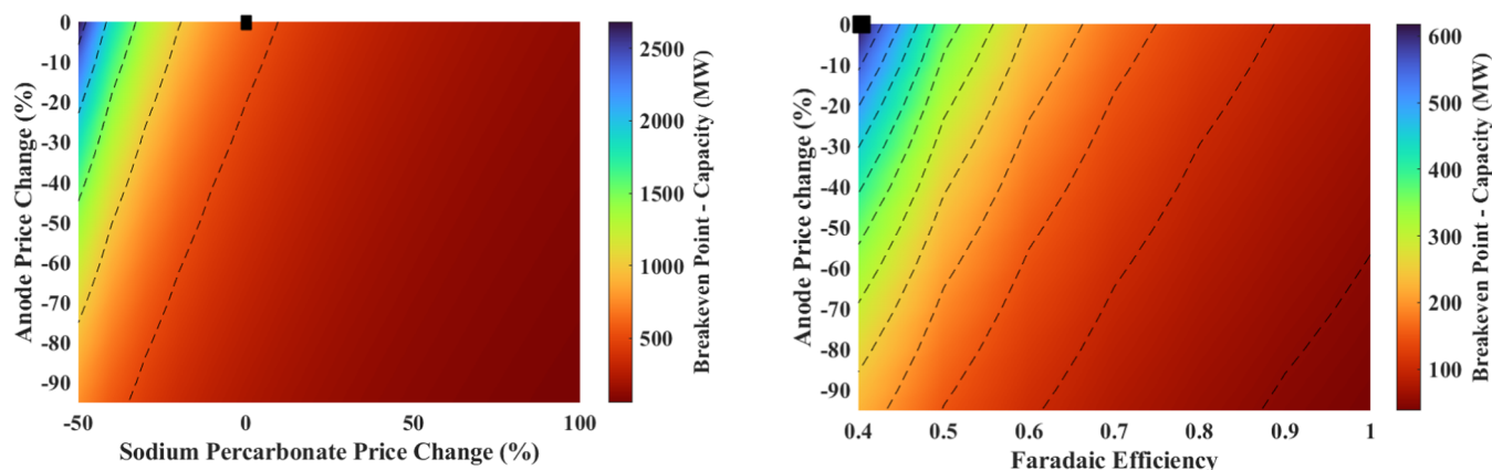
Figure 17. Effect of changes in the sodium percarbonate price and the anode price on the breakeven point (black marker shows the current situation).
