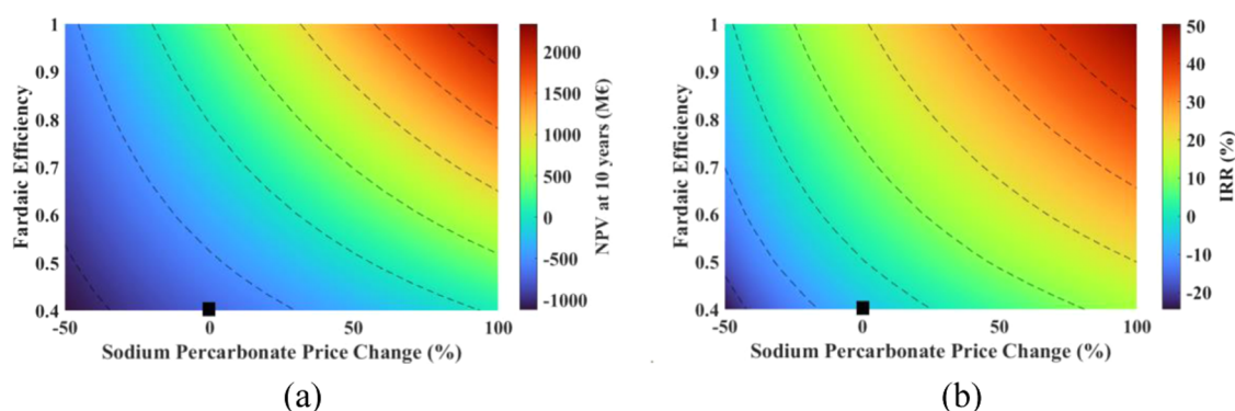
Figure 16. Effect of changes in the sodium percarbonate price and the Faradaic efficiency on (a) NPV, and (b) IRR (black marker shows the current situation).
