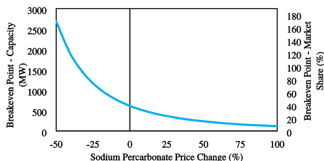
Figure 7. Effect of the SPC price on the breakeven point.
