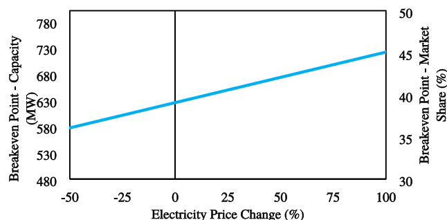
Figure 4. Effect of the electricity price on the breakeven point.
