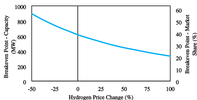
Figure 8. Effect of the hydrogen price on the breakeven point.
