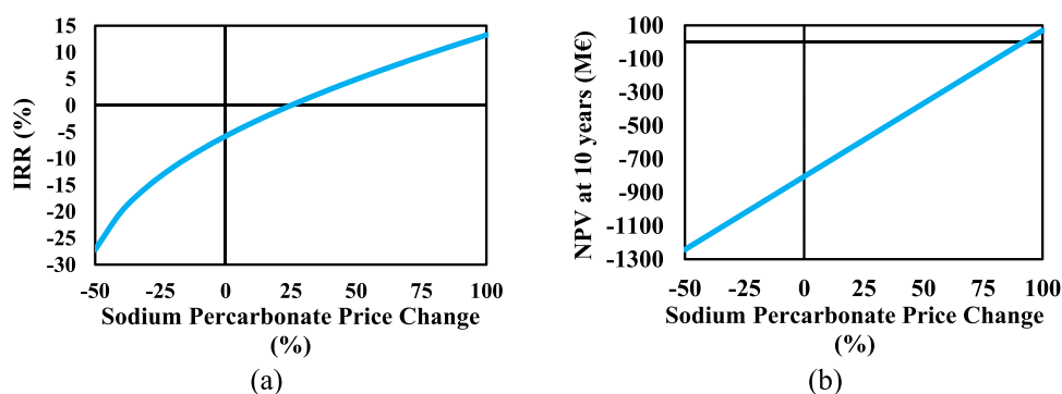
Figure 12. Effect of the sodium percarbonate price on (a) IRR, and (b) NPV.
