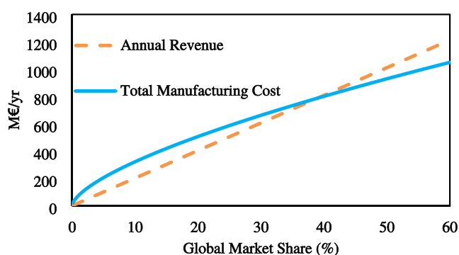
Figure 2. Breakeven point analysis based on a six-tenths heuristic for scaling the plant capacity.
