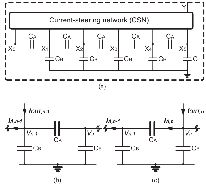
Fig. 6. (a) Capacitive ladder feedback network with CSN to realize the variable gain. Arbitrary section of the ladder network, with a feedback connection to (b) node n - 1 and (c) node n .
