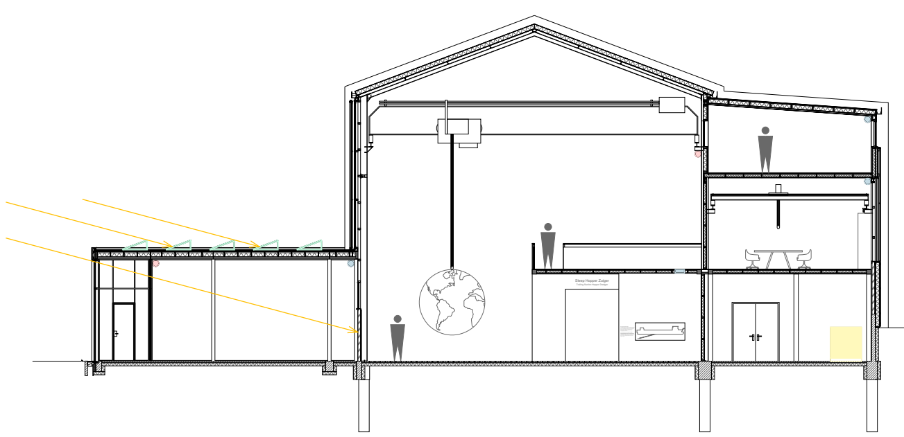
KO Winter Section 1:200
