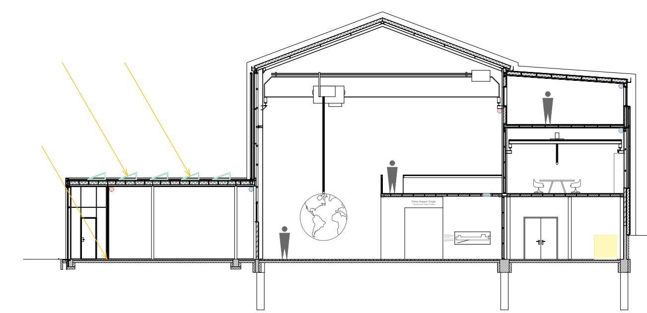
KO Summer Section 1:200
