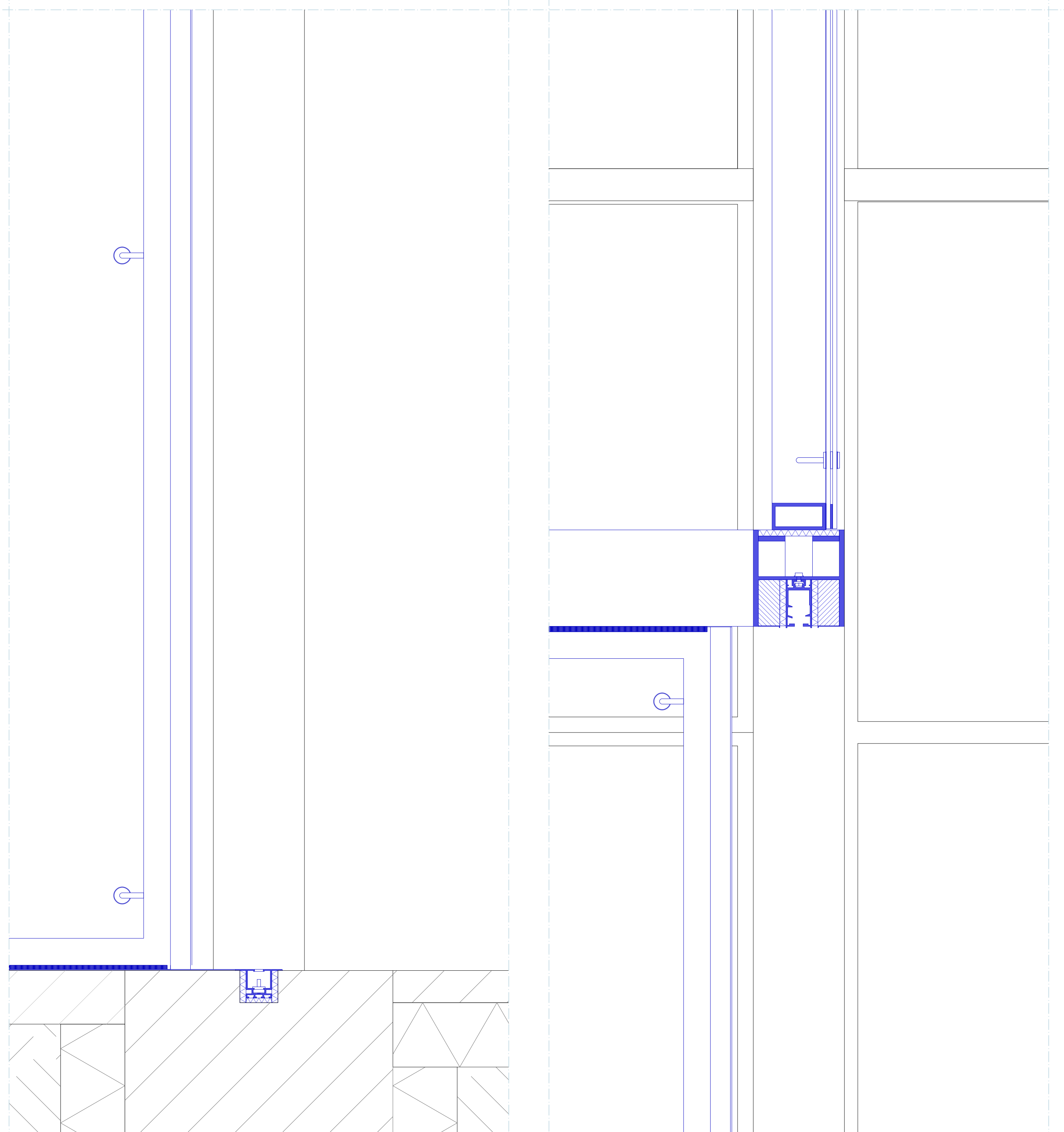
4&5. Vertical Details 1:5
