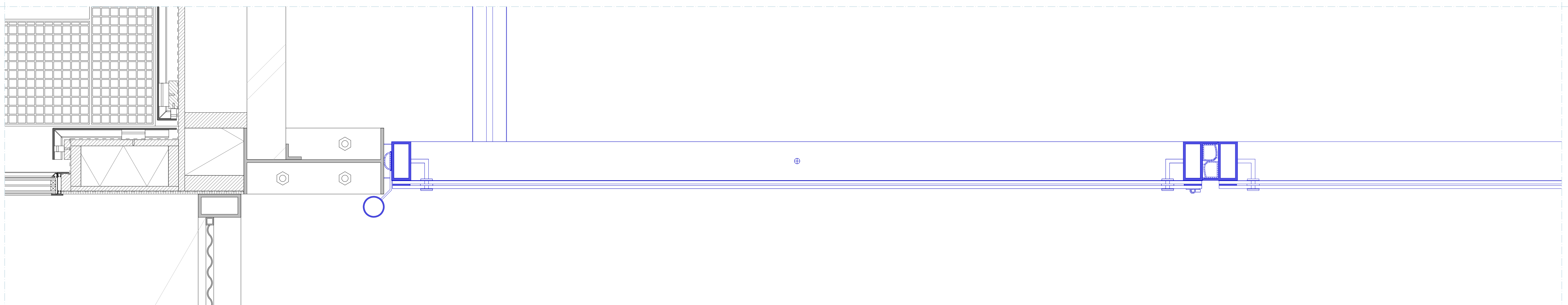
1. Horizontal Detail 1:5
