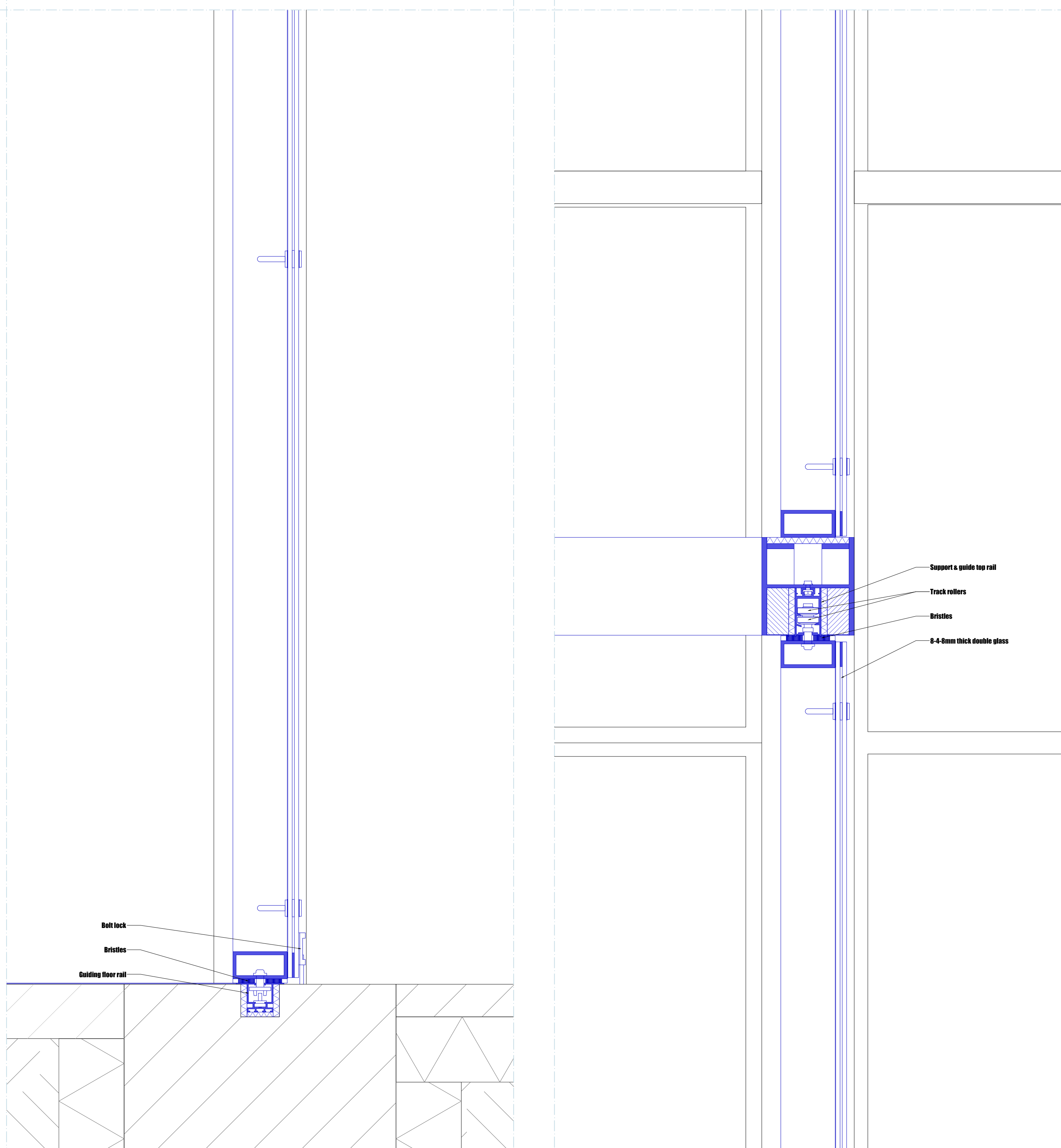
2&3. Vertical Details 1:5
