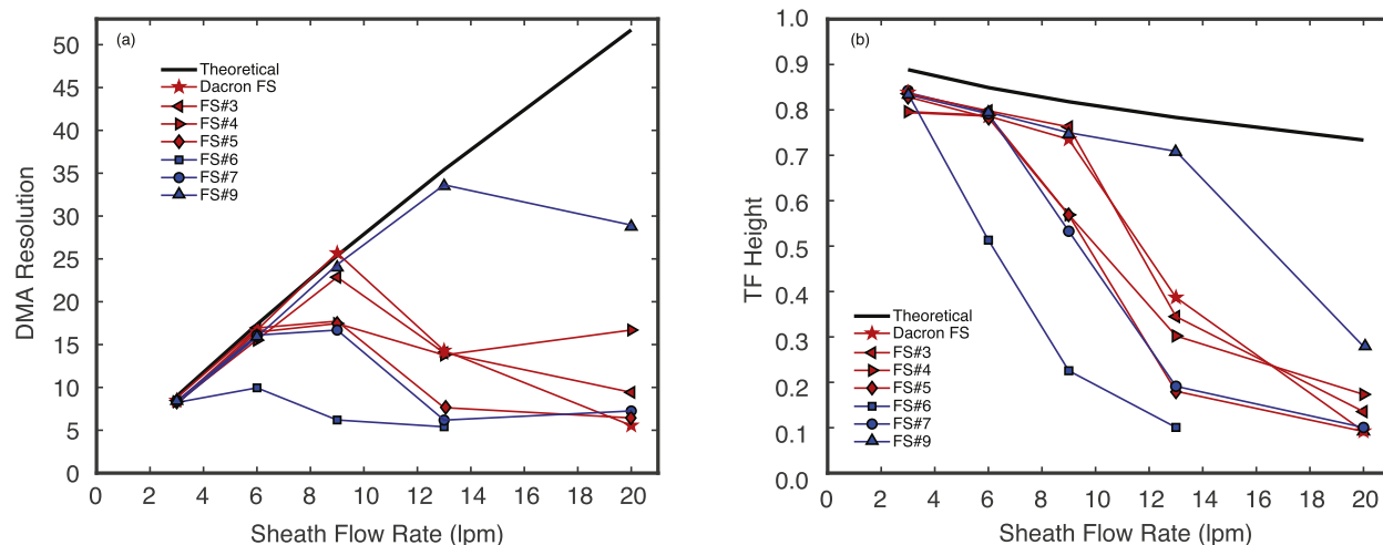
Fig. 3. DMA resolution (a) and TF height (b) of the test DMA (i.e., DMA-2 in the setup shown in Fig. 2) as a function of the sheath flow rate and when different FSs were employed.
