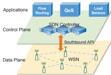
Fig. 1. Architecture of software-defined wireless sensor networks (SD-WSN).
