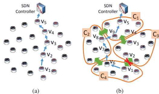
Fig. 2. (a) The communication flow is managed by each nodes. (b) The SD-WSN controller inserts cluster-level routing rules.
