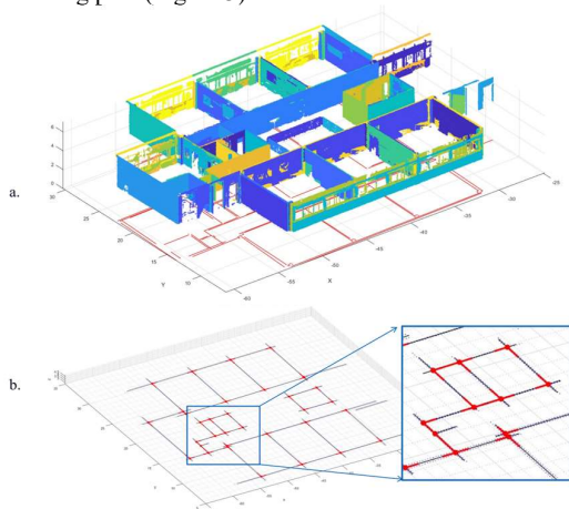
Figure 2. Definition of the Topological Map : a) lines extraction from a point cloud; b) the Topological Map with Intersection Key points J (red points) and directional vectors \mathcal{V} (red arrows).
