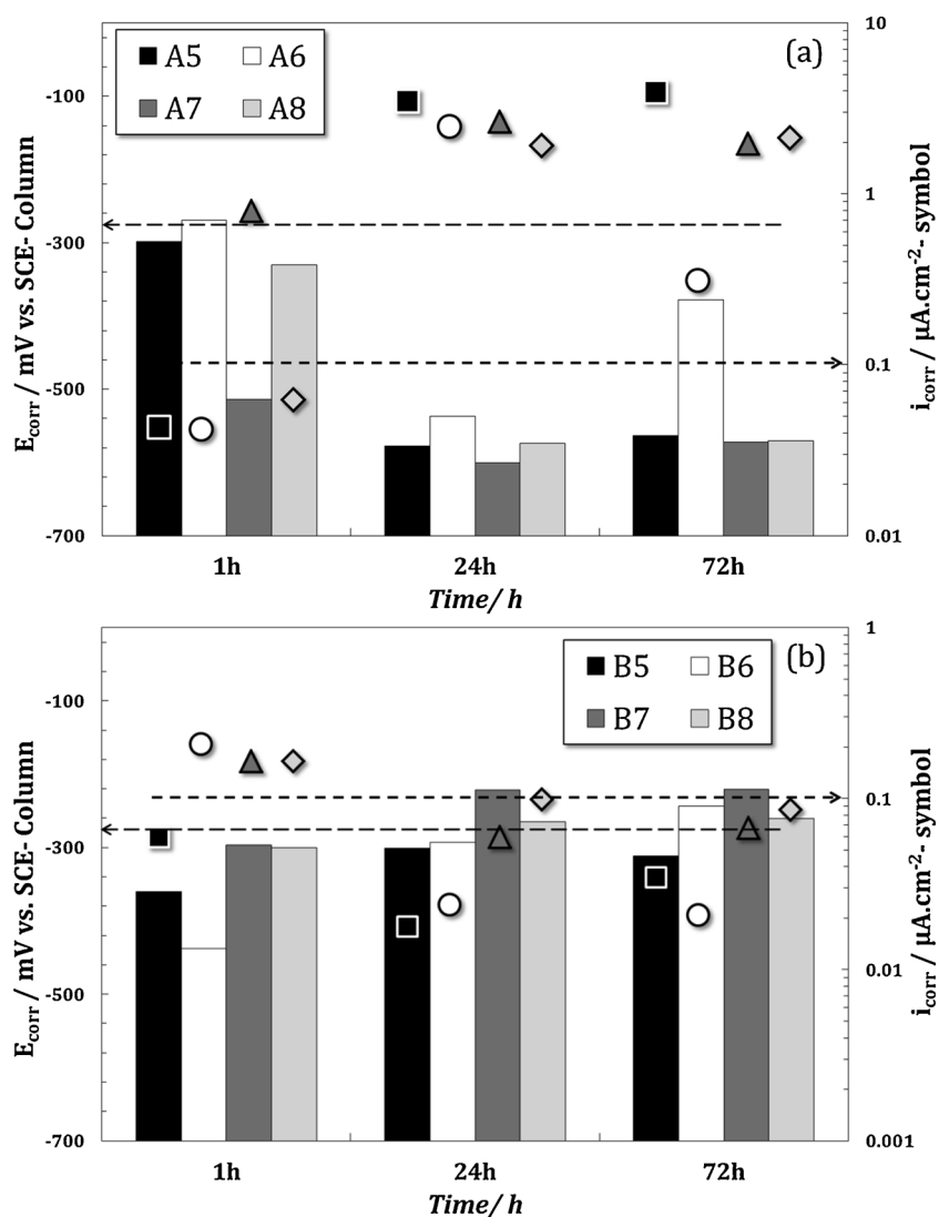
Fig. 3. Corrosion potential ( E_{\text{corr}} , columns) and corrosion current density ( i_{\text{corr}} , symbols) for steel in chloride-containing solutions: (a) 0.1 M NaOH (A5–A8); (b) 0.9 M NaOH (B5–B8).
