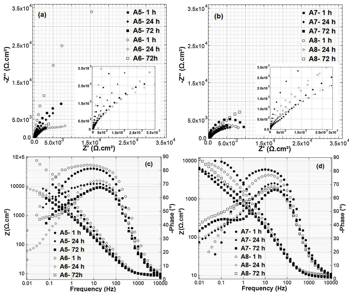
Fig. 8. Overlay of Nyquist (a,b) and Bode (c,d) diagrams of carbon steel after 1, 24 and 72 hours of immersion in chlorid-containing A5–A6 and A7–A8 solutions.
