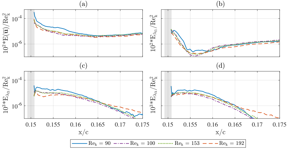
FIGURE 5.9: Variation of (a) E(\bar{u}) , and E_{\lambda_{fi}}(\bar{u}) computed for FFT modes (b) \lambda_{f1} , (c) \lambda_{f2} and (d) \lambda_{f3} modes at varying Re_k . Energy is scaled by Re_k^2 ; element location (grey shaded region).
