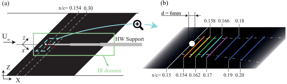
FIGURE 2.8: (a) Sketch of HWA experimental set-up and coordinate reference systems (not to scale). Y-axis and y-axis are directed towards the reader, HWA measurement domain (light blue rectangle), IR measurement domain (green rectangle). (b) Zoomed-in sketch of HWA acquisition yz planes in the element vicinity (dashed blue region in (a)).
