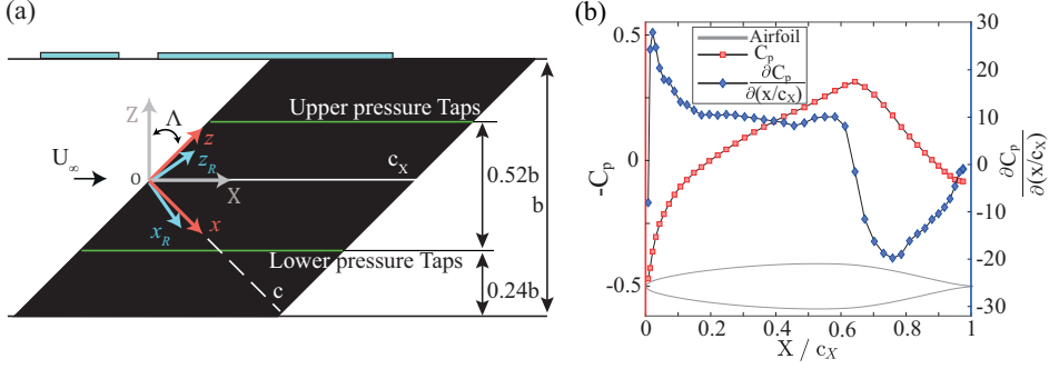
FIGURE 2.1: (a) M3J swept wing diagram with coordinate systems: tunnel-attached (grey, XYZ ); wing-attached (red, xyz ); CF vortex aligned (light blue x_R y_R z_R ). Y -axes, y -axes and y_R axes are all directed towards the reader. Light-blue rectangles represent windows cut in the tunnel ceiling. (b) M3J airfoil geometry (aligned to the freestream direction X ), pressure coefficient and pressure gradient distribution measured by the lower and upper arrays of pressure taps at \alpha = -3.36^\circ , Re_{c_X} = 2.17 \times 10^6 .
