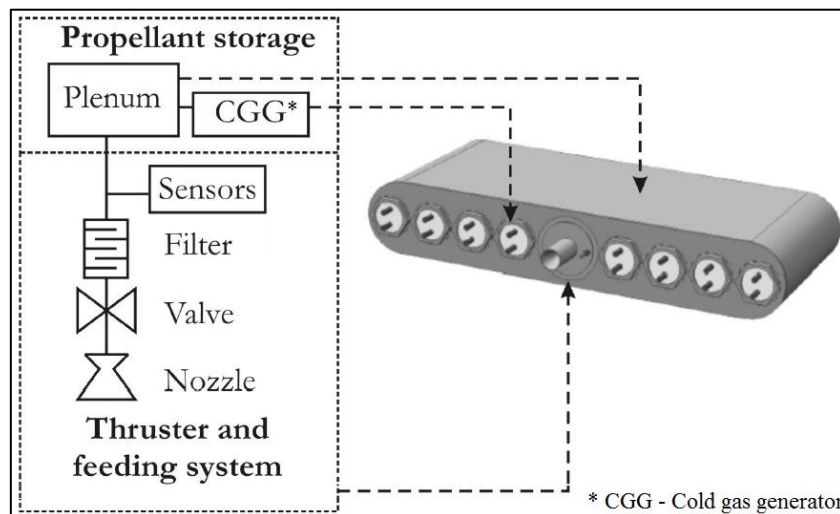
10 Figure 3 – Example of cold-gas thruster (adapted from [51]) designed for the Delfi-N3xt mission.
