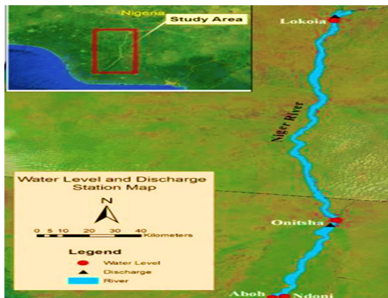
Figure 3.5. Dredging data coverage area on the Niger River. Onitsha water level data is used for model calibration
