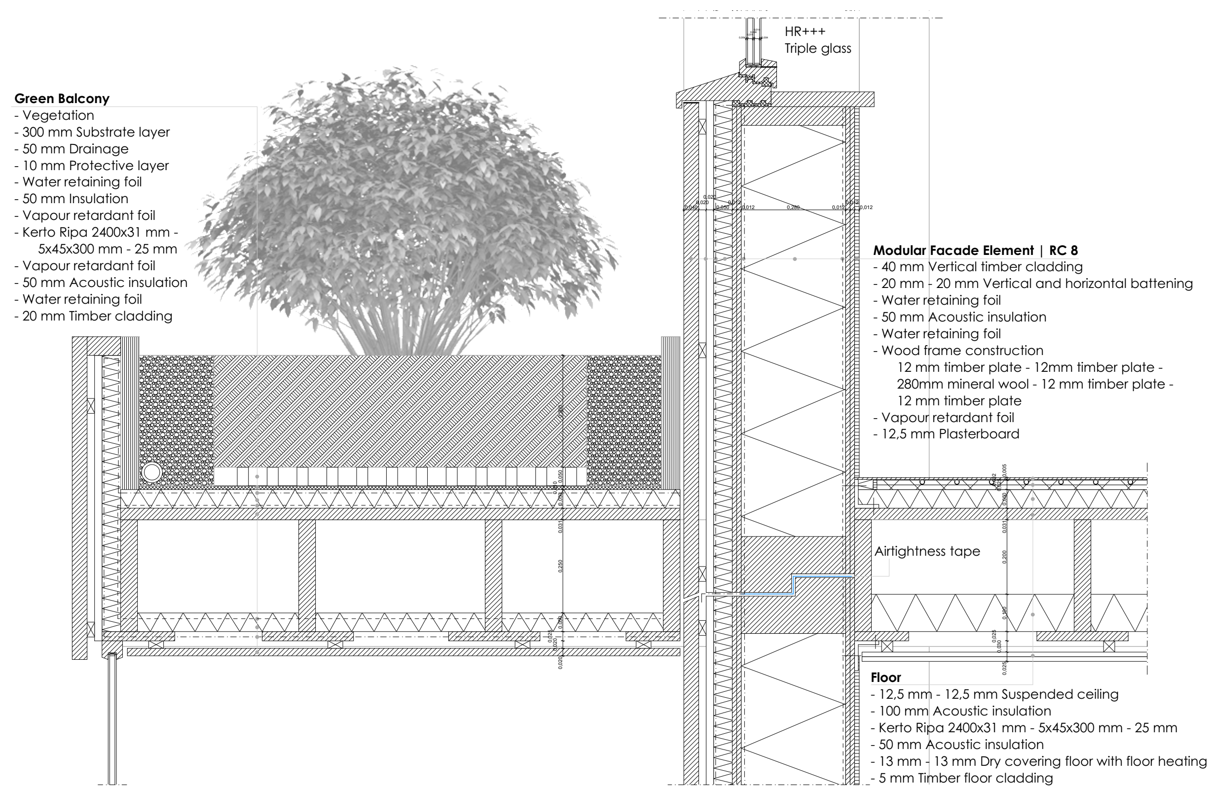
Green Balcony Vertical Detail 1:10
