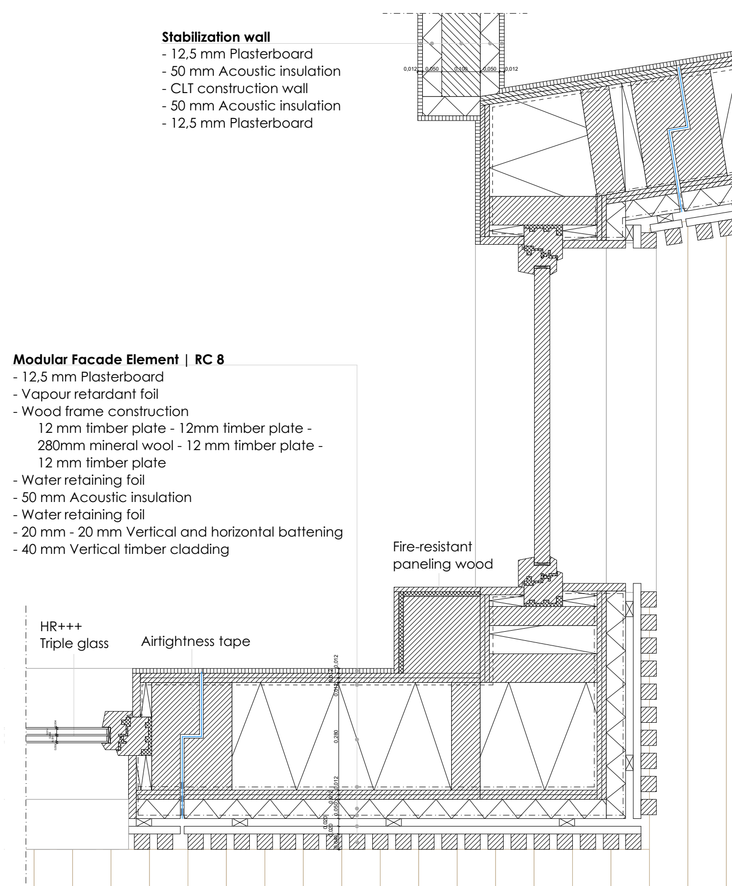
Horizontal Detail 1:10
