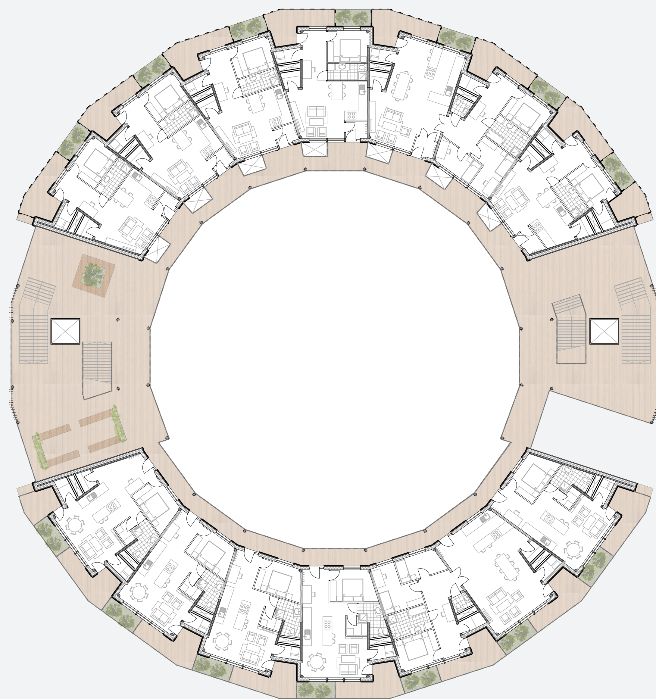
Floorplan Second Floor 1:200
