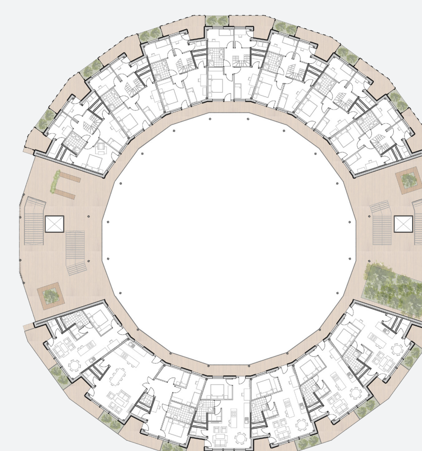
Floorplan First Floor 1:500
