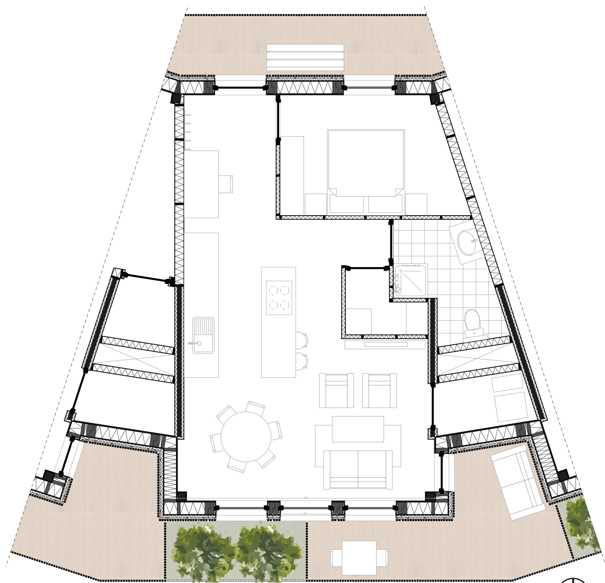
Floorplan North Entrance Apartment 1:50
