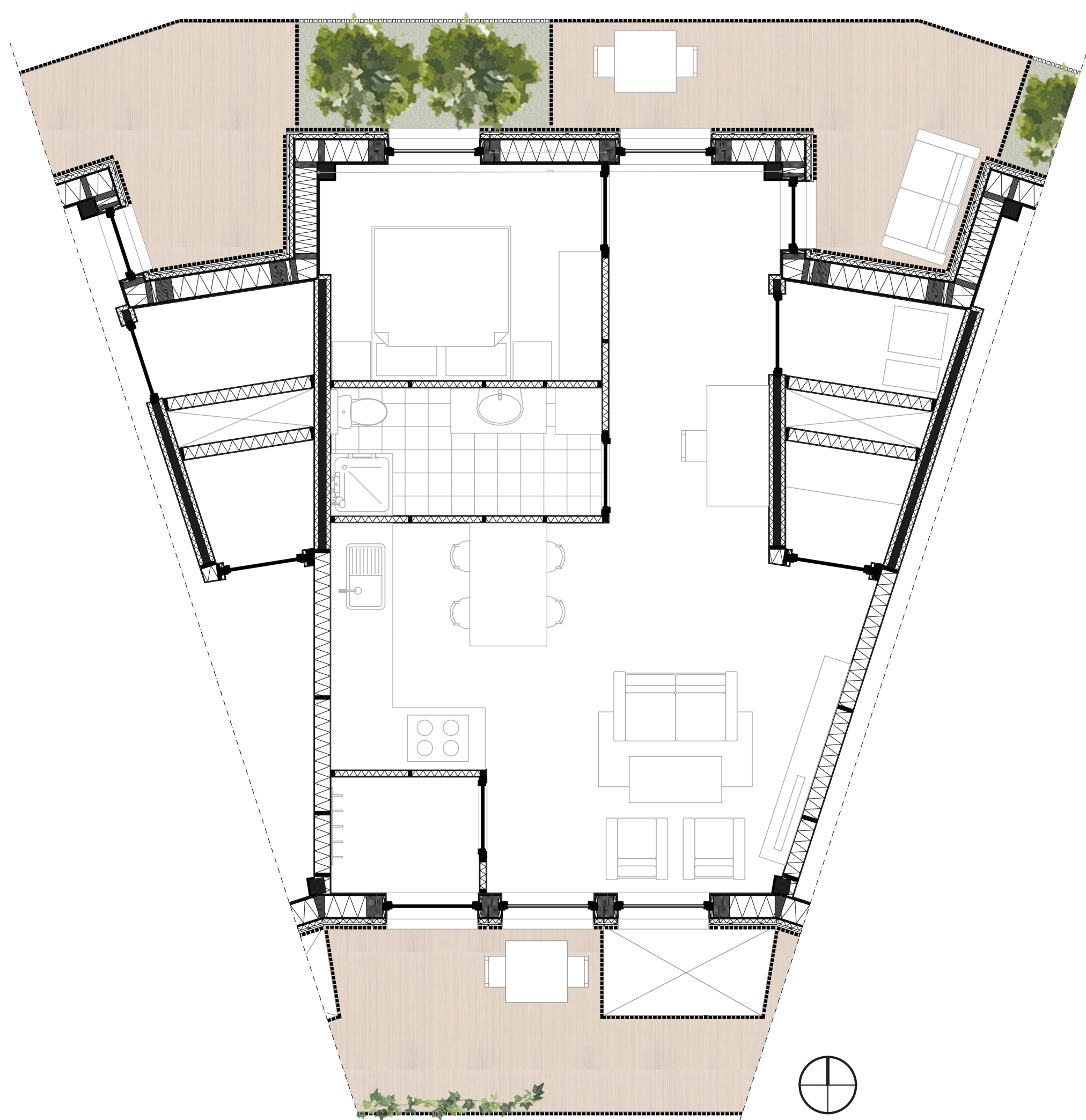
Floorplan South Entrance Apartment 1:50
