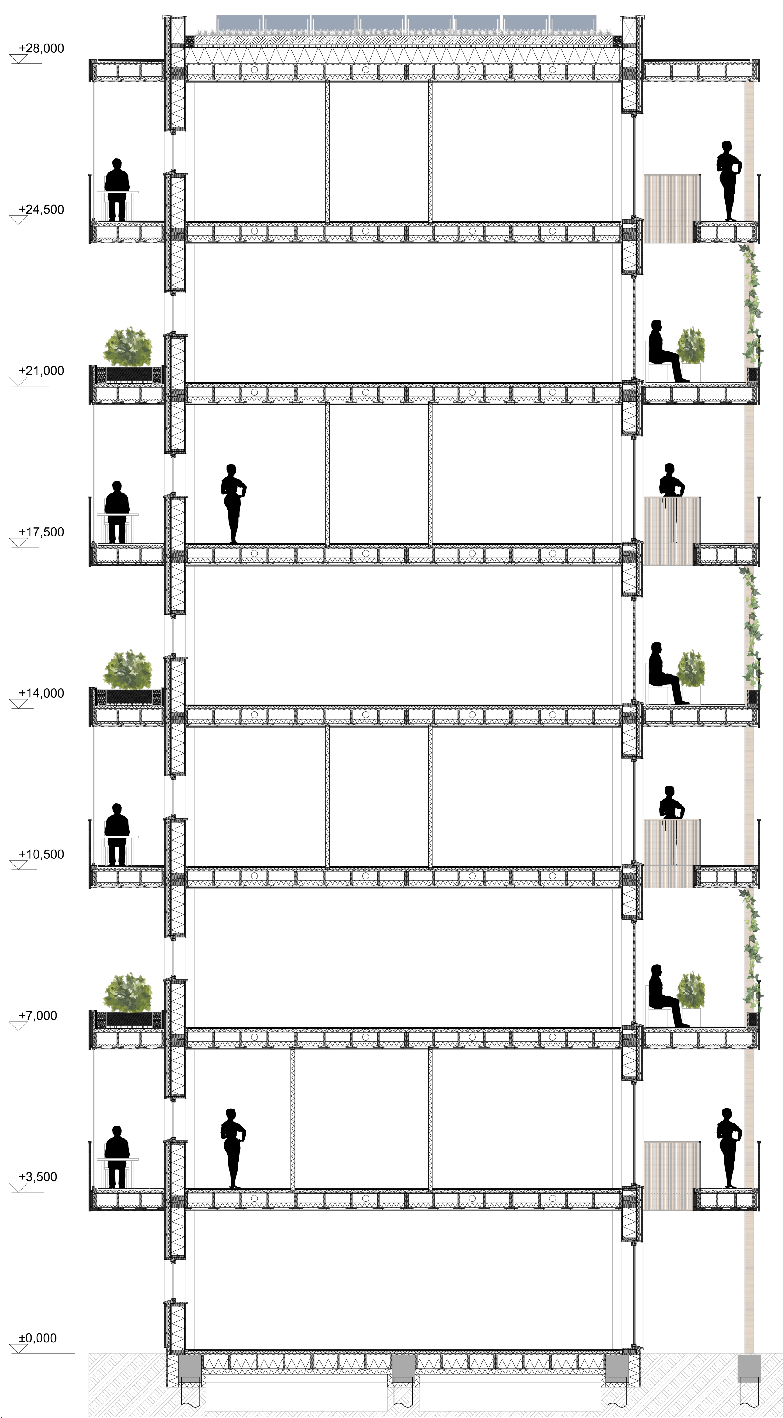
Facade Fragment 1:50
