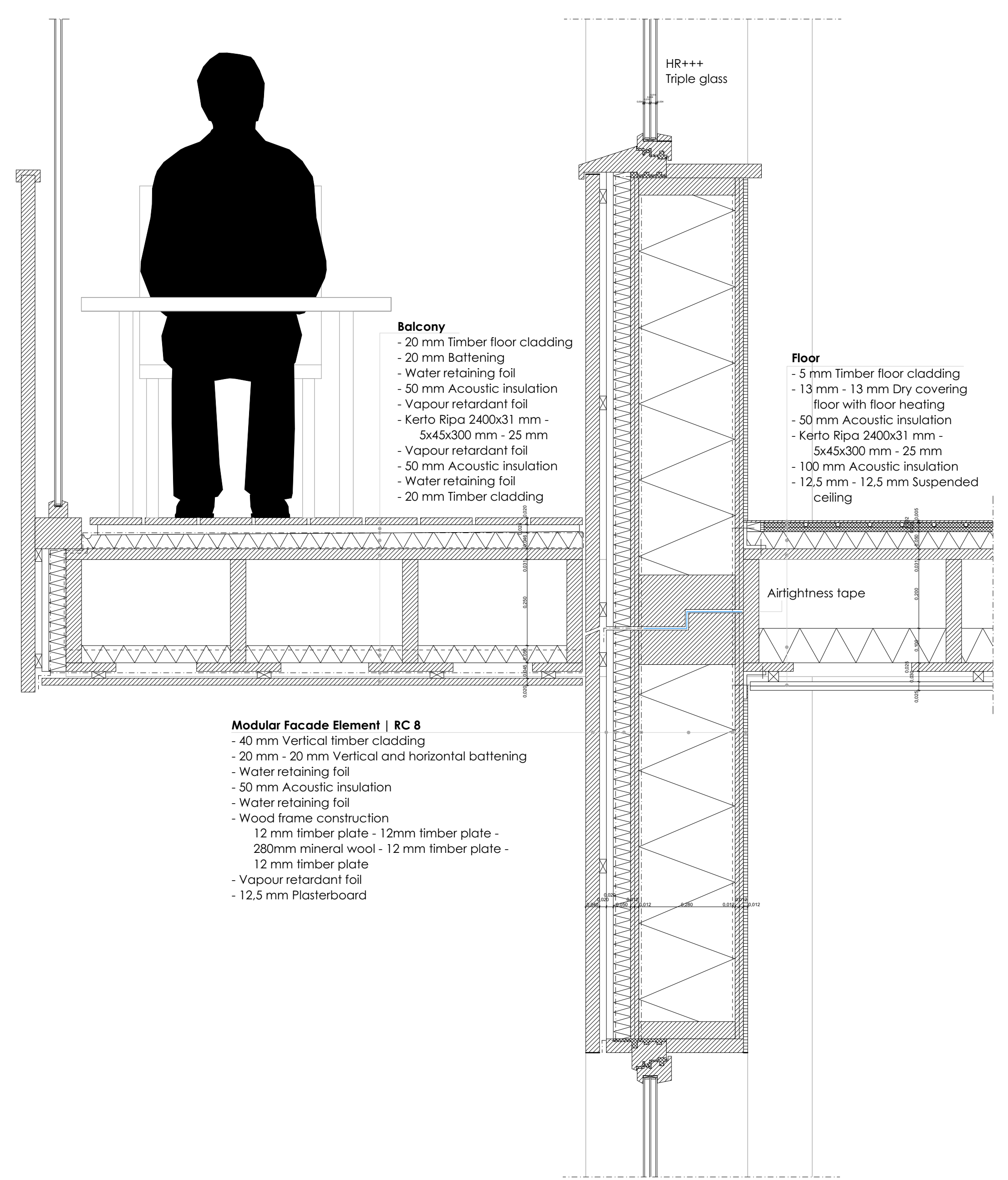
Balcony Vertical Detail 1:10
