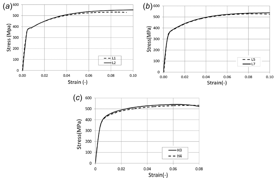
Fig. 9 The material stress–strain relationship from tensile tests: (a) coupons L1 and L2, (b) coupons L5 and L7, and (c) coupons H3 and H4
