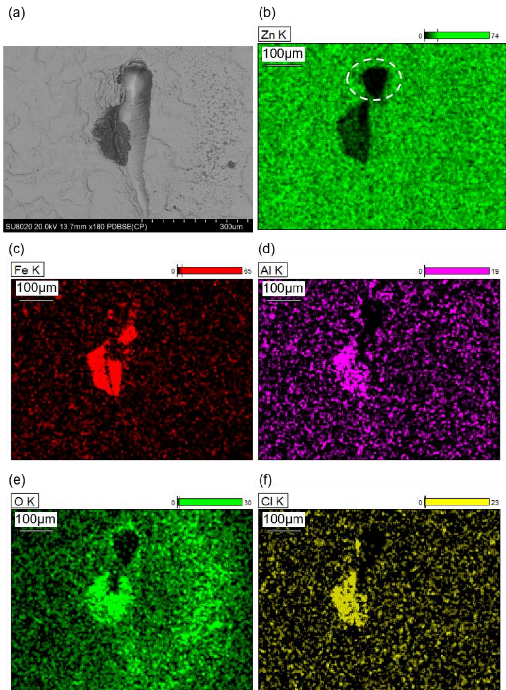
Fig. 9. SEM-EDX analysis of the moderately scribed HDG surface ( \sim 12 \mu\text{m} -defect depth) after 180 min of immersion in 0.05 M NaCl electrolyte. (a) Backscattered electron image electron image. (b, c, d, e, f) Corresponding EDX elemental maps of Zn, Fe, Al, O and Cl.
