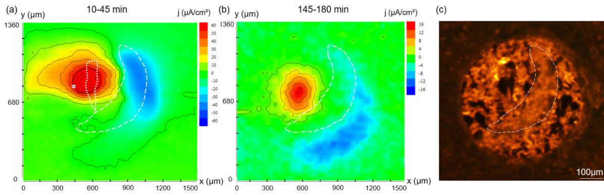
Fig. 8. Current density ( \mu\text{A}/\text{cm}^2 ) maps obtained by SVET from HDG presenting a partially scribed Zn coating exposed to 0.05 M NaCl solution. Scans were obtained between (a) 10-45 min and (b) 145-180 min of immersion. The scratched zone is represented by white dots in (a). (c) the corresponding optical micrograph taken after 180 min. The dashed lines in (a), (b) and (c) delimit the region with intense precipitation of white corrosion products.
