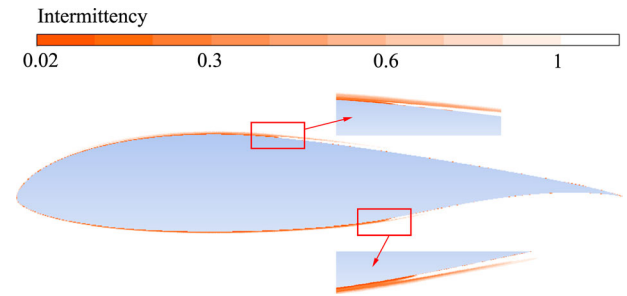
Figure 8 Intermittency contours at Re = 4 \times 10^6
