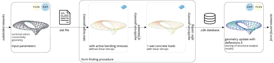
Fig. 8. Form finding of gridshell.
