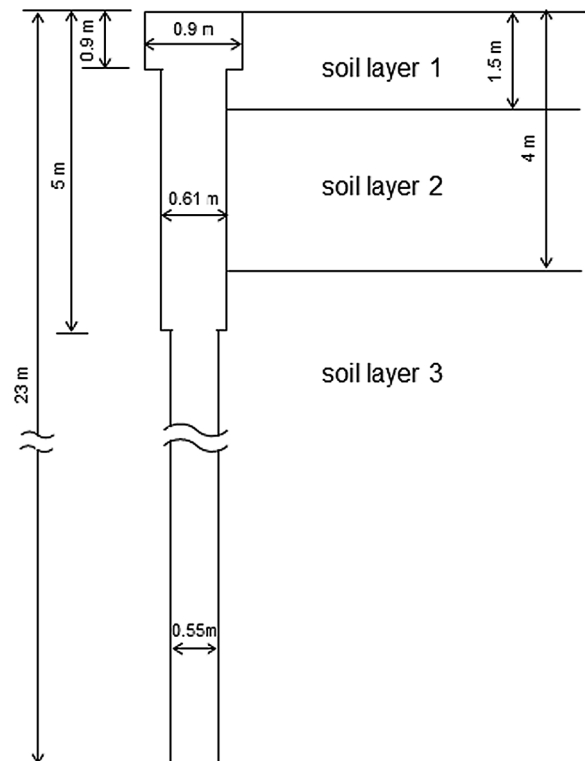
Fig. 5. London energy pile geometry.
