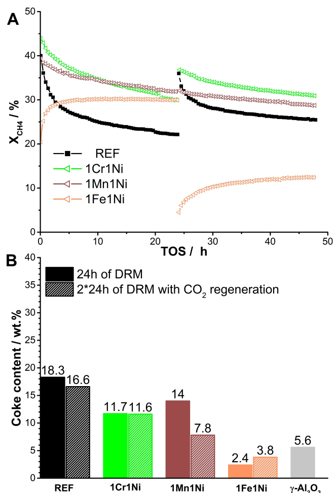
Figure 10. Conversion (A) and coke content (B – solid symbols 24 h of reaction, shaded symbols 2*24 h and regeneration) before and after regeneration with CO 2 for the samples 1X1Ni (10 mg sample, 650 °C, 100 mL min -1 of 25% CH 4 , 25% CO 2 in N 2 ).
