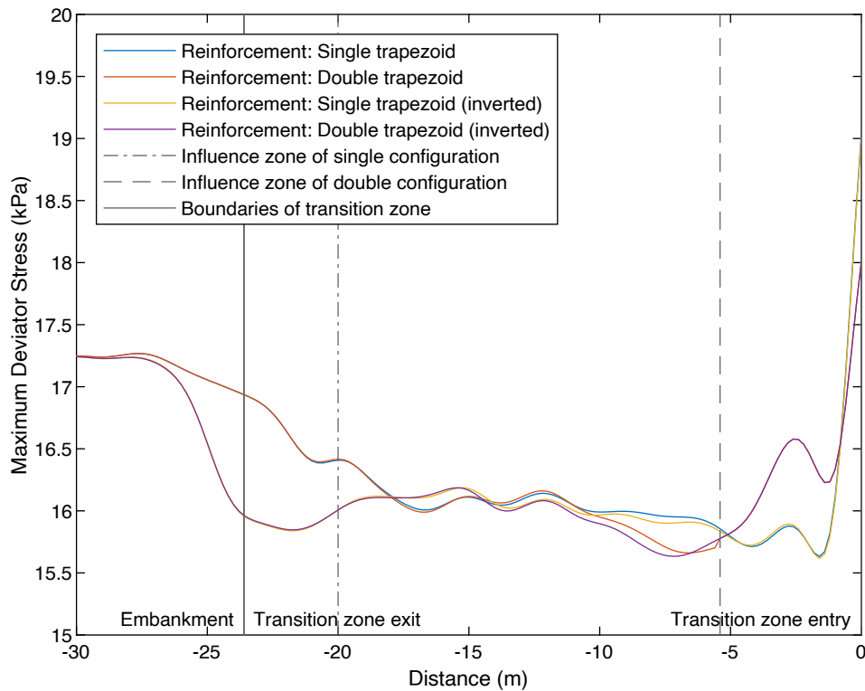
Fig. 17. Subbase deviator stress for different earthwork configurations supporting the ballasted track.
