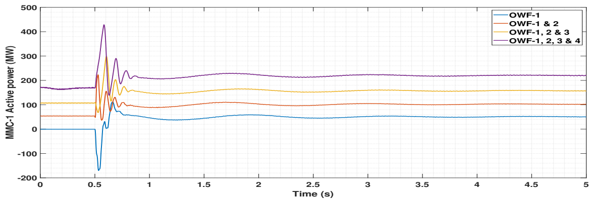
Figure 22. Active power in MMC-1 bus upon connecting all OWFs with 50 MW generation each.
