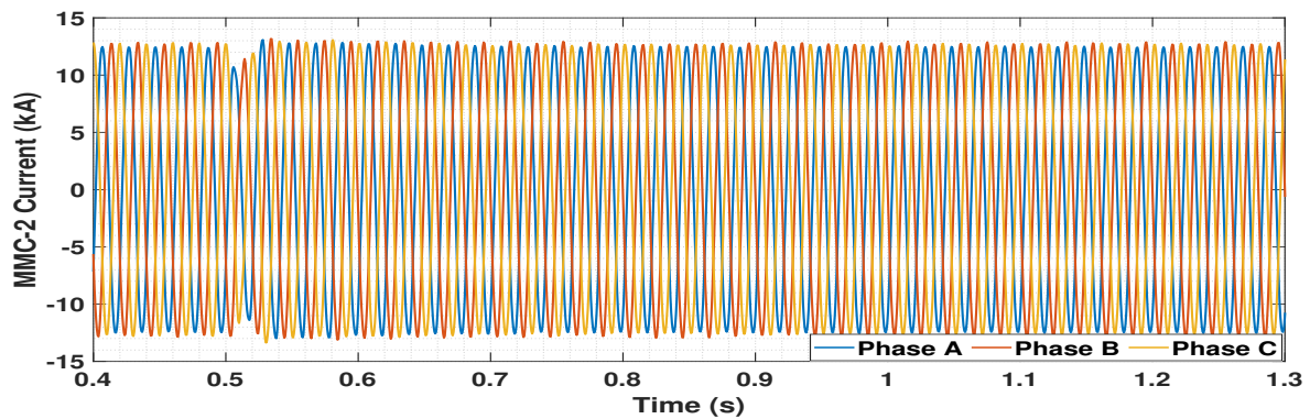
(b) Currents in MMC-2 bus
