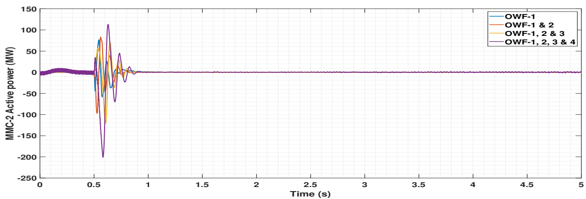
Figure 23. Active power in MMC-2 bus upon connecting all OWFs with 50 MW generation each.
