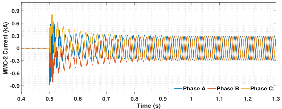
(b) Currents in MMC-2 bus
