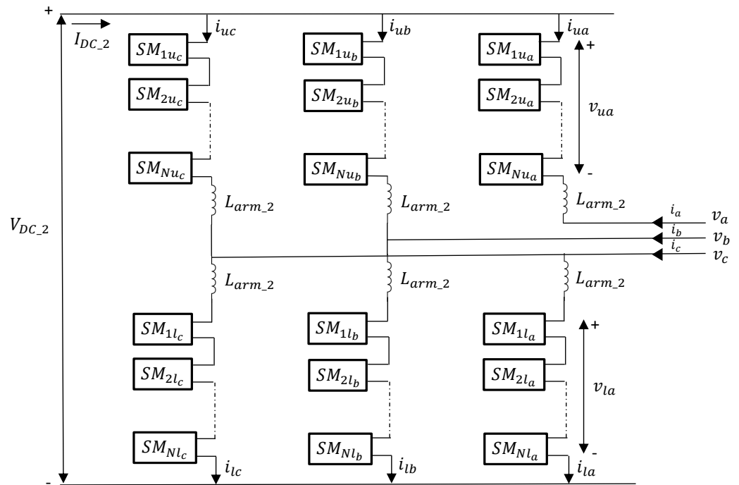
Figure 10. MMC-2 representation.
