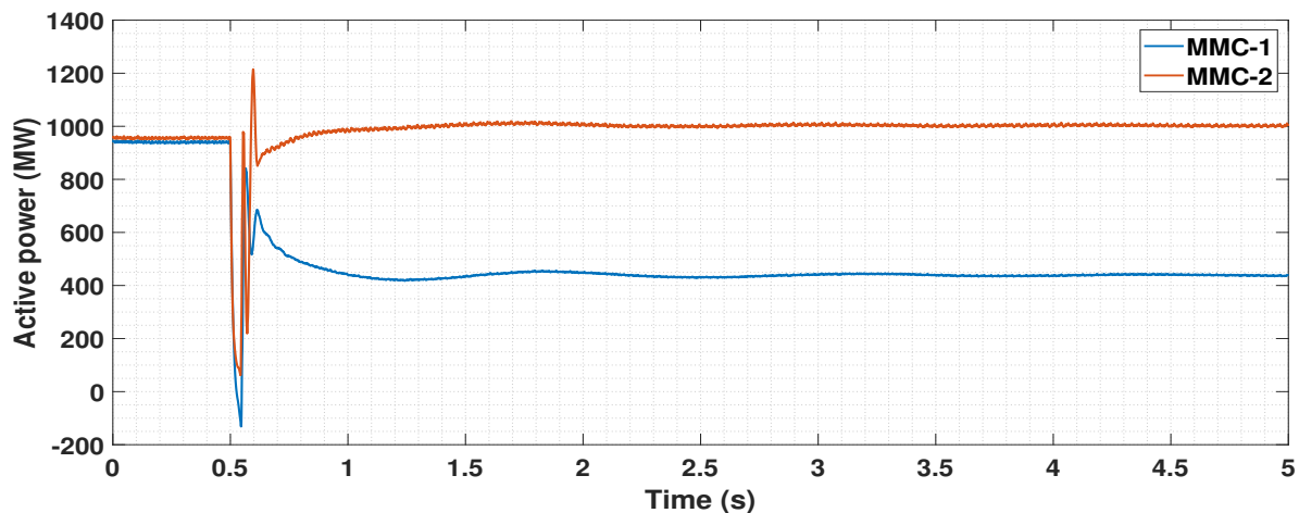
Figure 32. Active power in MMC-1 bus and MMC-2 bus upon three-phase line to ground fault in the middle of cable-1.
