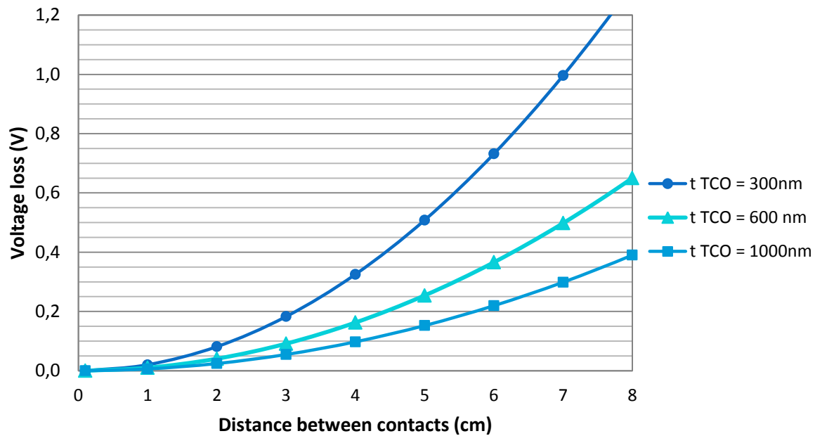
Figure 55. Voltage loss due to sheet resistance at the TCO layer for different travel lengths and film thicknesses
