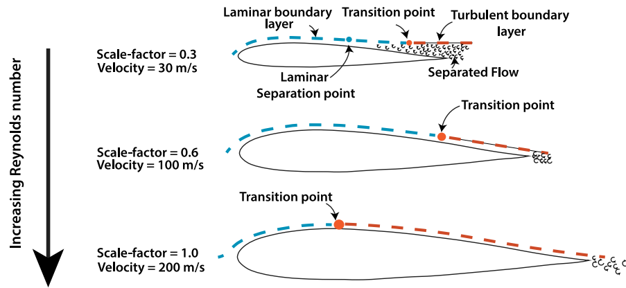
Fig. 17. Geometrically scaled models do not guarantee geometrically scaled shapes of the boundary layer. This is because the model scales as per euclidean geometry whereas the flow-field does not [137]. Here, the 30% scaled model has completely different flow characteristics as compared to the prototype due to separation. In case of 60% scaled model, the streamlines have similar shapes but different transition point, which must be corrected to predict prototype behaviour.
