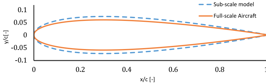
Fig. 25. The transformation of airfoil shape necessary to maintain similar pressure distribution in inviscid flow between a sub-scale model tested at 0.3 Mach and the full-scale aircraft tested at 0.65 Mach.
