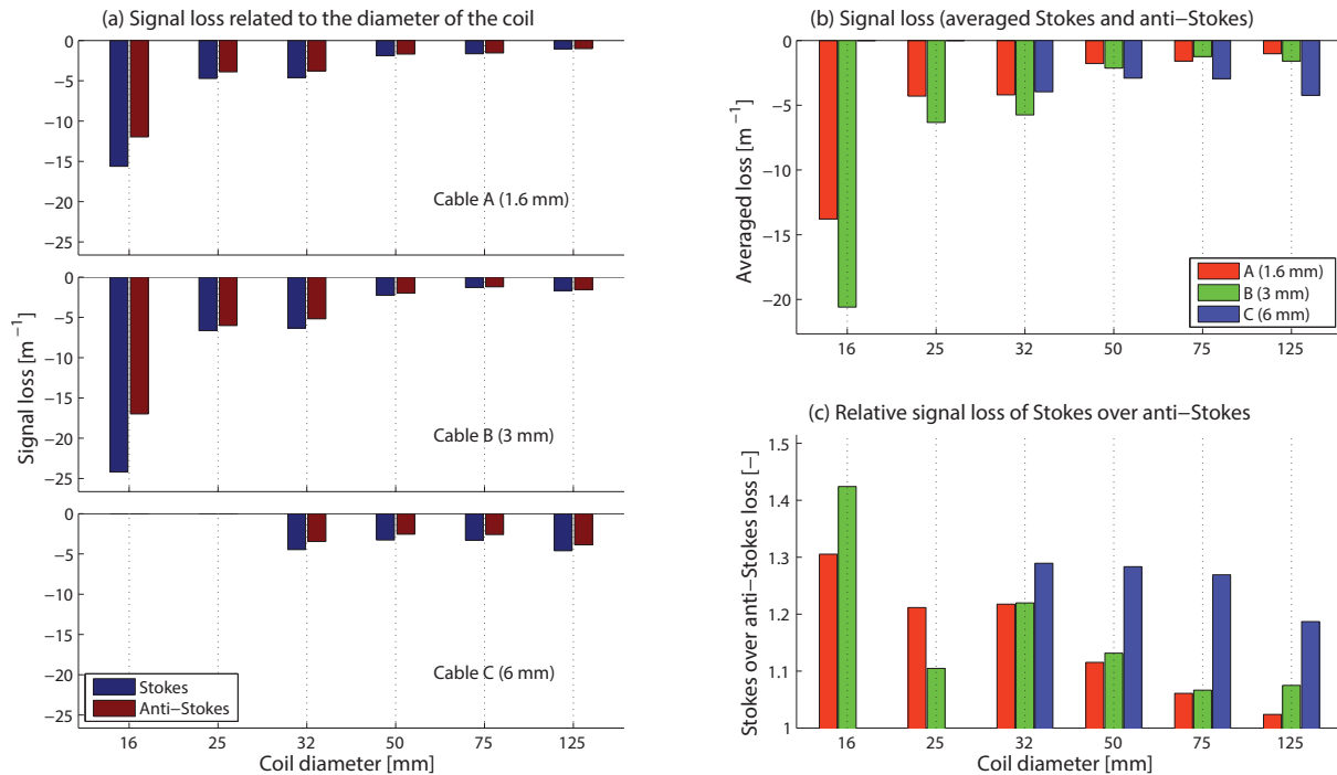
Figure 6. (a) Stokes and anti-Stokes signal loss ( \text{m}^{-1} ) for coil diameters of 16, 25, 32, 50, 75, and 125 mm, and for the cables A, B, and C (from top to bottom). (b) Combination of the bar plots in the left pane using the average of the Stokes and anti-Stokes signals. Loss decreasing with increasing diameter is indicative of bend-related light loss, which is generally associated with differential loss as a function of light frequency. (c) Ratio of Stokes over anti-Stokes losses as a function of coil diameter.
