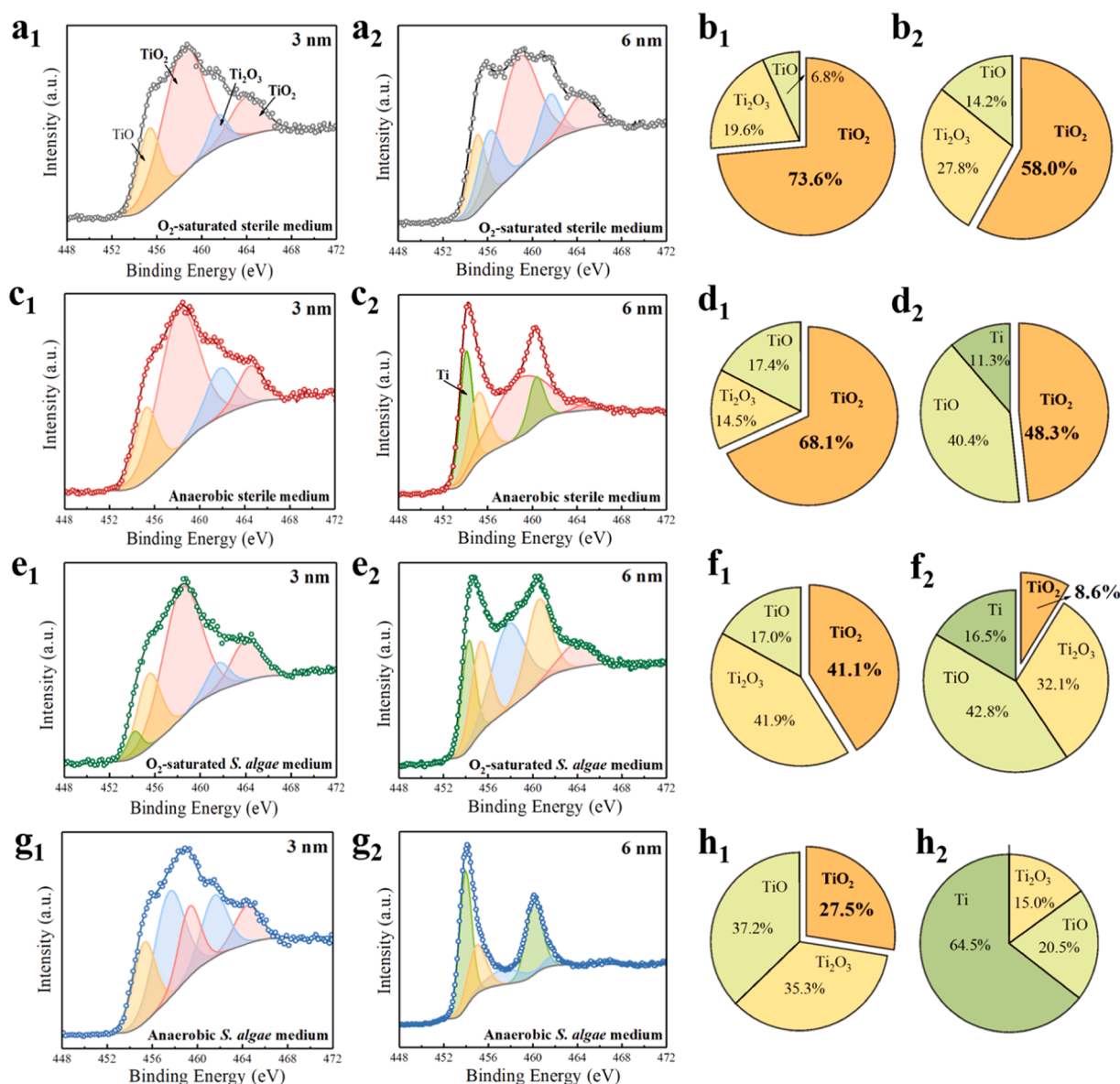
Fig. 8. Detailed XPS spectra at 3 nm/6 nm and cation percentages of Ti 2p peaks after incubation for 14 days in the different medium: (a 1 , a 2 , b 1 , b 2 ) O 2 -saturated sterile medium, (c 1 , c 2 , d 1 , d 2 ) anaerobic sterile medium, (e 1 , e 2 , f 1 , f 2 ) O 2 -saturated S. algae medium and (g 1 , g 2 , h 1 , h 2 ) anaerobic S. algae medium.
