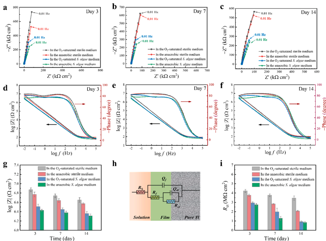
Fig. 5. The Nyquist and Bode raw plots of Ti coupons exposed to the different mediums after (a, d) day 3, (b, e) day 7 and (c, f) day 14. g the \log |Z| values at 0.01 Hz of coupons exposed to the different mediums. h Equivalent fitting circuit. The equivalent circuit model is composed of the electrolyte resistance ( R_s ), the oxide layer resistance or the mixture resistance of oxide layer and biofilm ( R_f ), the charge-transfer resistance ( R_{ct} ), the capacitive properties of the oxide layer ( Q_f ) and the capacitive properties of electric double-layer capacitance at the film/solution interface ( Q_{dl} ). i The R_{ct} value from EIS data fitting. Results are the mean and standard deviation ( n > 3 ). Error bars represent standard deviations from at least three independent coupons.
