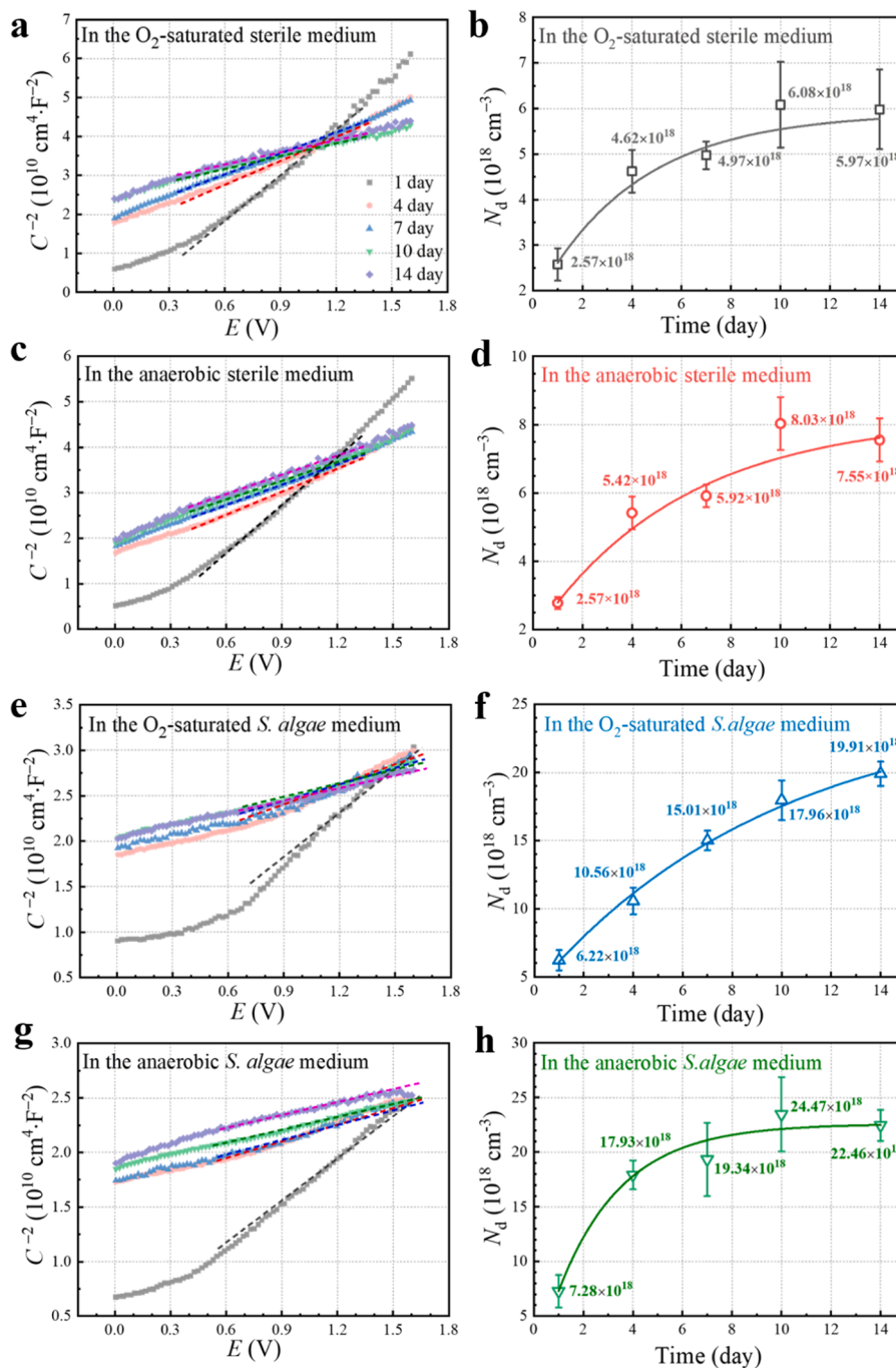
Fig. 9. Mott-Schottky plots and the variations of fitted donor densities after different days: (a, b) in the sterile medium of O 2 -saturated culture solutions and (c, d) anaerobic culture solutions, (e, f) in the presence of S. algae of O 2 -saturated culture solutions and (g, h) anaerobic culture solutions. The dots are experimentally measured data and the lines are the fitting curves. Results are the mean and standard deviation ( n > 3 ). Error bars represent standard deviations from at least three independent coupons.
