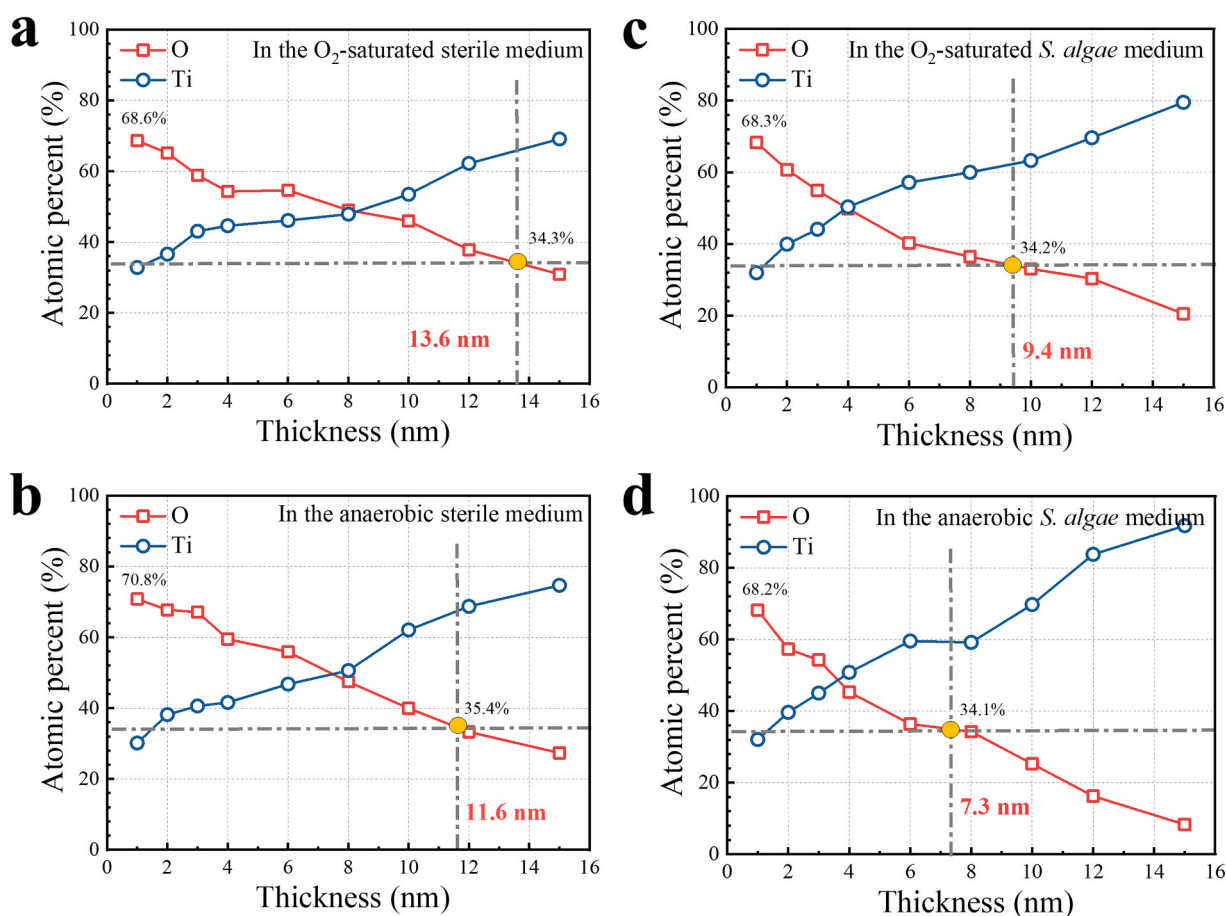
Fig. 7. Depth profiles of the passive films formed on the Ti immersed in the different media after 14 days: a in the sterile medium of O 2 -saturated culture solutions and b anaerobic culture solutions, c in the presence of S. algae of O 2 -saturated culture solutions and d anaerobic culture solutions. Results are the mean and standard deviation ( n > 3 ). Error bars represent standard deviations from at least three independent coupons.
