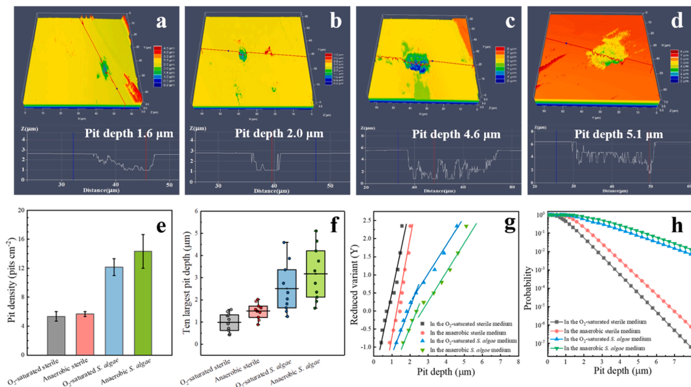
Fig. 6. CLSM 3-D images for the deepest pits on Ti after immersion of 14 days: a in the sterile medium of O 2 -saturated culture solutions and b anaerobic culture solutions, c in the presence of S. algae of O 2 -saturated culture solutions and d anaerobic culture solutions. e Statistics of pitting density. f Ten largest pit depths in the different culture media after 14 days of incubation. Statistics of pit depth: g Gumbel probability plots for the pit depth and h probability of various pits of Ti in the different mediums.
