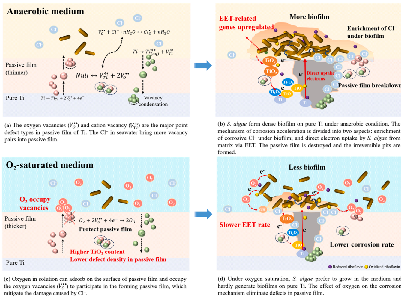
Fig. 11. Mechanistic diagrams showing the effect of DO and S. algae on corrosion of commercially pure Ti.
