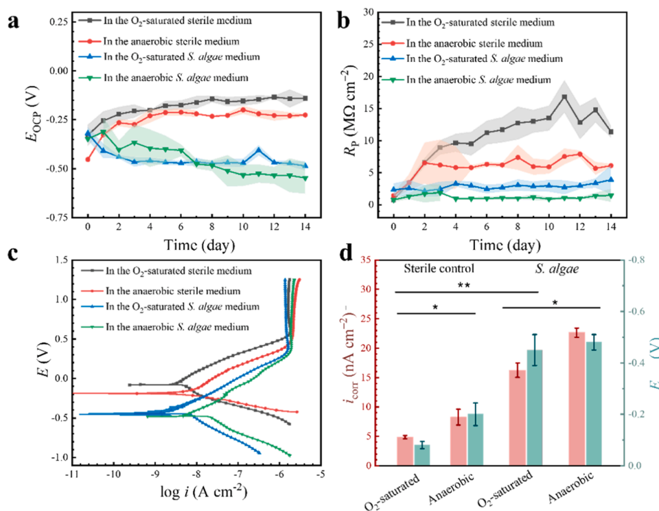
Fig. 4. Corrosion behavior of Ti in the different media: Variations of a E_{OCP} and b R_p data over time, c potentiodynamic polarization curves of the samples after immersion for 14 days, and d fitted i_{corr} and E_{corr} values. Error bars represent standard deviations from at least three independent coupons. An asterisk represents a statistically significant difference (* p < 0.05 , ** p < 0.01 ).
