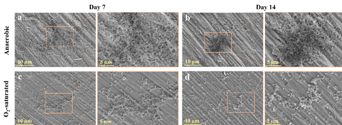
Fig. 1. SEM observation of S. algae biofilms attached on the Ti coupon surface in the anaerobic culture solutions at a Day 7 and b Day 14, in the O 2 -saturated culture solutions at c Day 7 and d Day 14.
